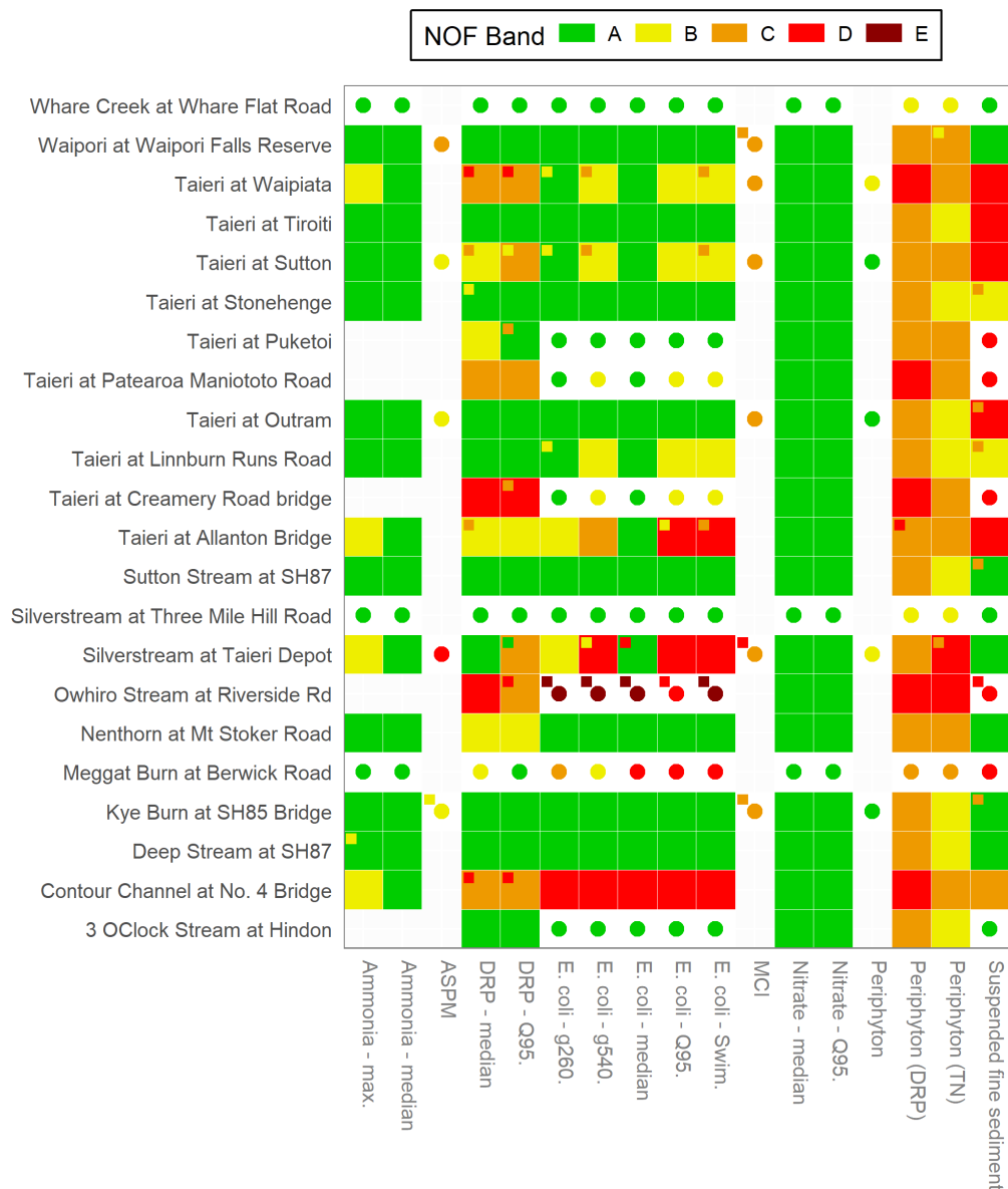
Figure 3 Grading of the river sites of the Taieri FMU based on the NOF criteria. Grades for sites that did not meet the sample number requirements in Table 4 are shown as white cells with coloured circles. The white cells indicate sites for which the variable was not monitored. Small square in the upper left quadrant of the cells indicate the site grade for the baseline
