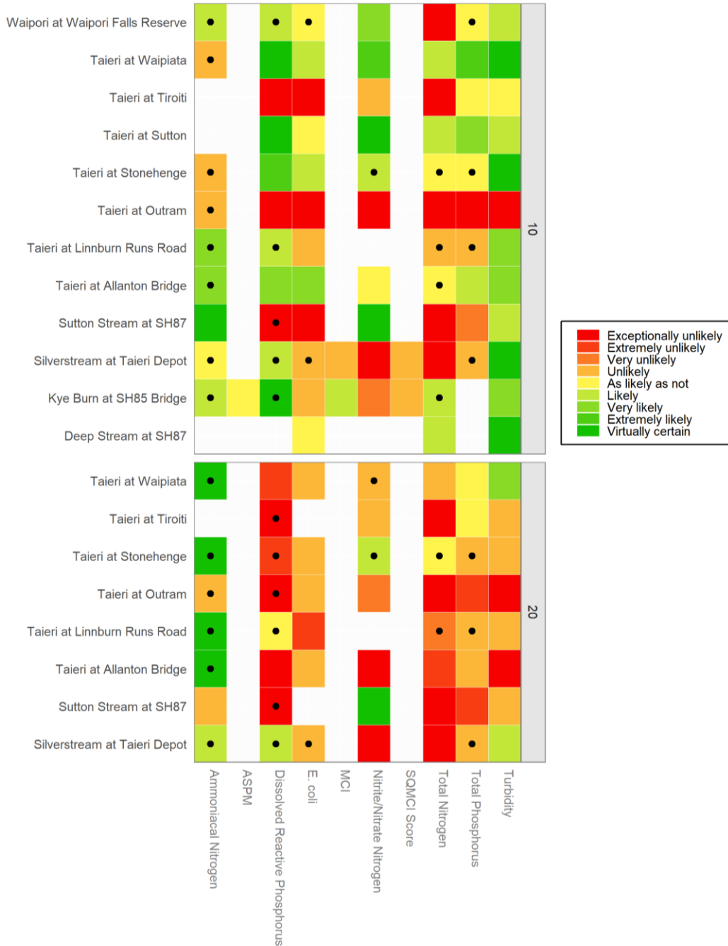
Figure 6 Summary of Taieri FMU river sites categorised according to the level of confidence that their 10 and 20 year raw water quality trends indicate improvement. Confidence that the trend indicates improvement is expressed using the categorical levels of confidence defined in Table 5. Cells containing a black dot indicate site/variable combinations where the Sen Slope was evaluated as zero (i.e., a trend rate that cannot be quantified given the precision of the
