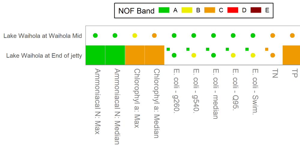
Figure 4 Grading of the lake sites of the Taieri FMU based on the NOF criteria. Grades for sites that did not meet the sample number requirements in Table 4 are shown as white cells with coloured circles. The white cells indicate sites for which the variable was not monitored. Small square in the upper left quadrant of the cells indicate the site grade for the baseline
