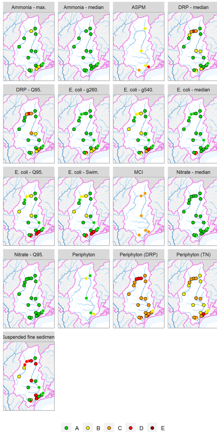
Figure 5 Maps showing Taieri FMU sites coloured according to their state grading as indicated by NOF attribute bands. Bands for sites that did not meet the sample number requirements specified in Table 4 are shown without black outlines
