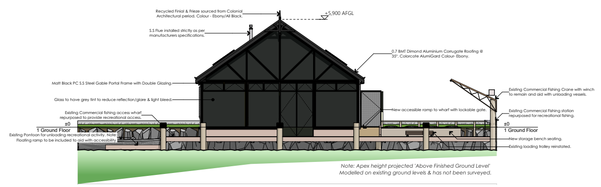
East Elevation
