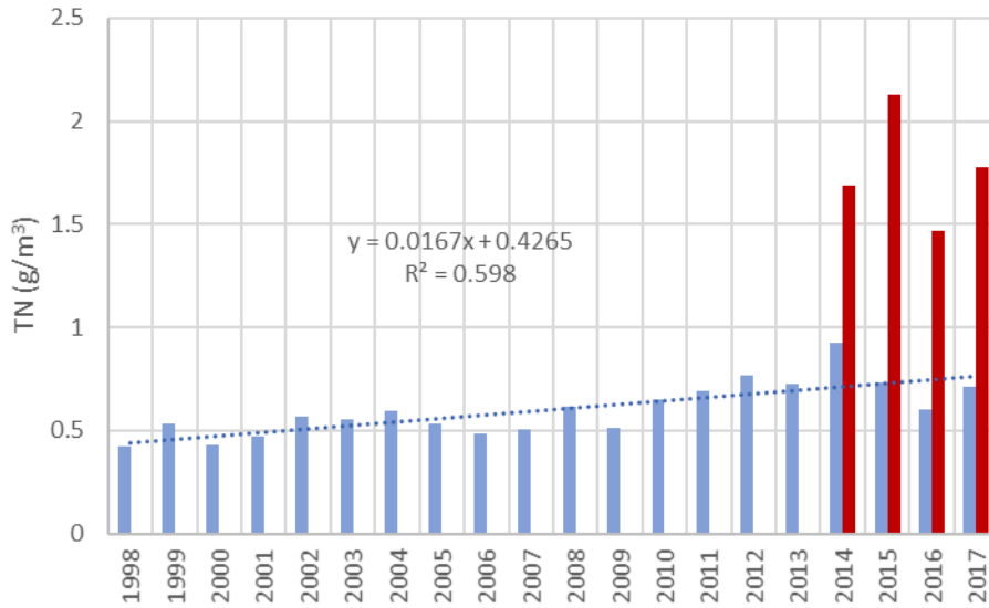
Figure 2-2: Mean annual total nitrogen concentrations in the Catlins River (blue) and Owaka River (red). Concentrations calculated from samples from Catlins@Houipapa and Owaka@Katea Rd.
