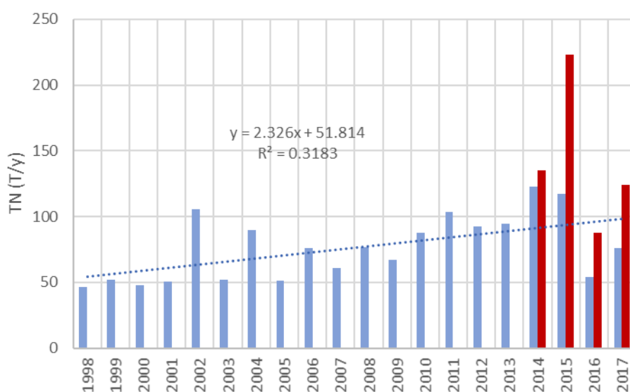
Figure 2-1: Annual total nitrogen loads from the Catlins River (blue) and Owaka River (red). Loads from the Catlins River calculated from daily flows and nutrient concentrations measured at Houipapa. Owaka River loads are calculated from daily flows and nutrient samples at Katea Road.
