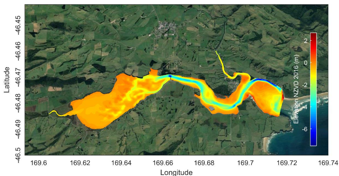
Figure 3-1: Surveyed bathymetry of the Catlins River Estuary. Bathymetry data compiled from surveys conducted 27–29 March 2018, and LIDAR data from 6–11 September 2004. Elevations are relative to NZVD 2016.
