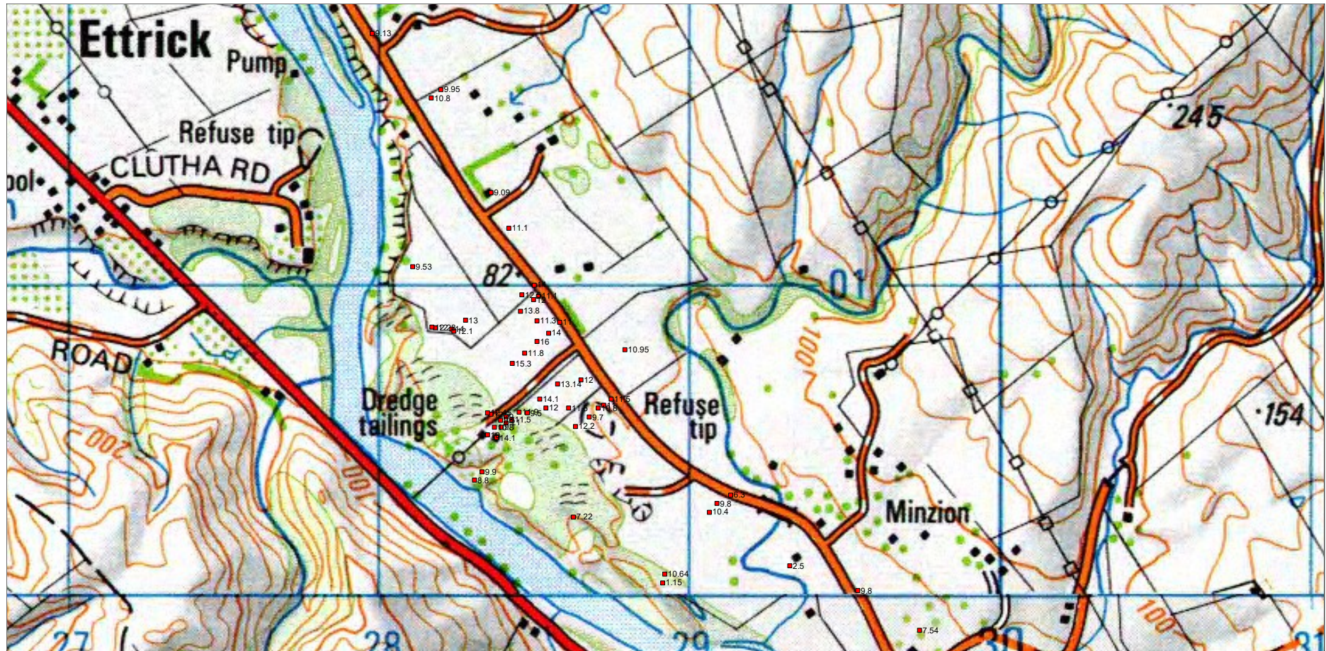
Depth to Water Table (m)
