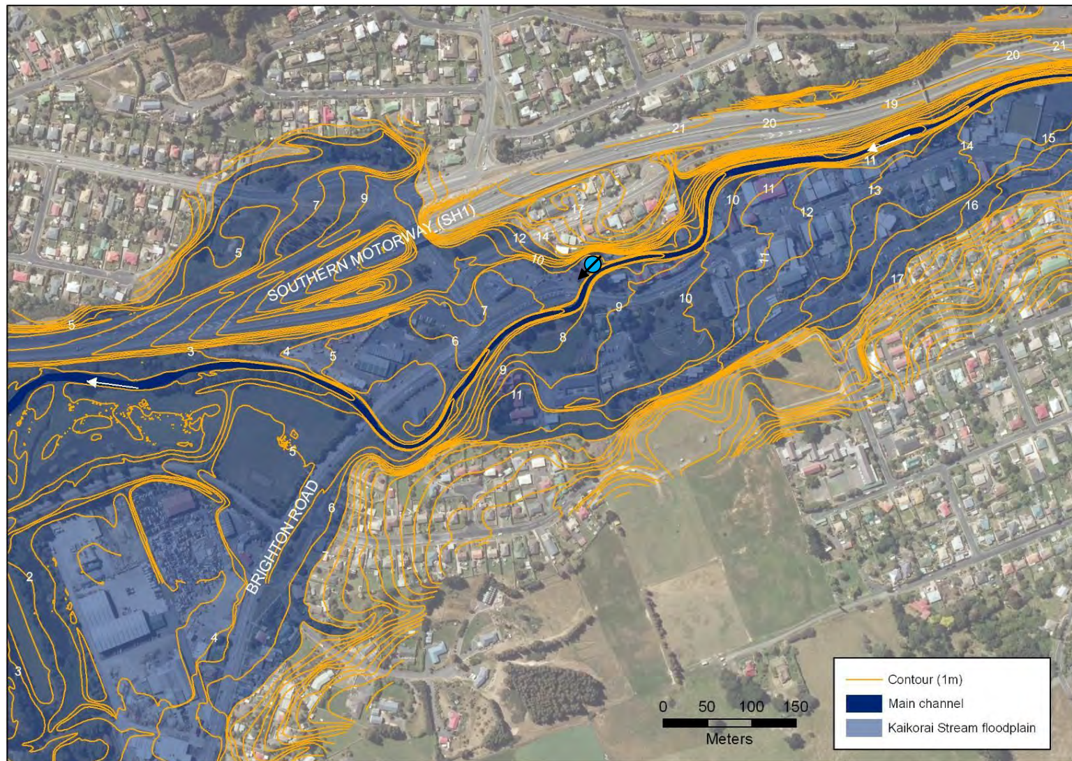
Figure 27 Kaikorai Stream floodplain area: Green Island to Brighton Road. The approximate direction and location of the photo shown in Figure 7 is also shown.
