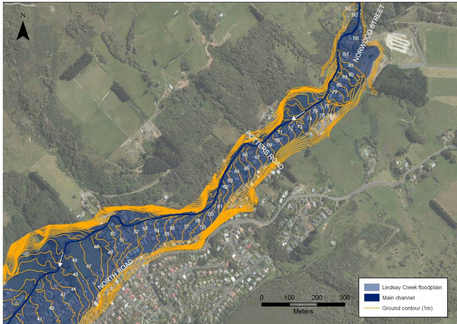
Figure 33 Lindsay Creek floodplain area - upper reach
