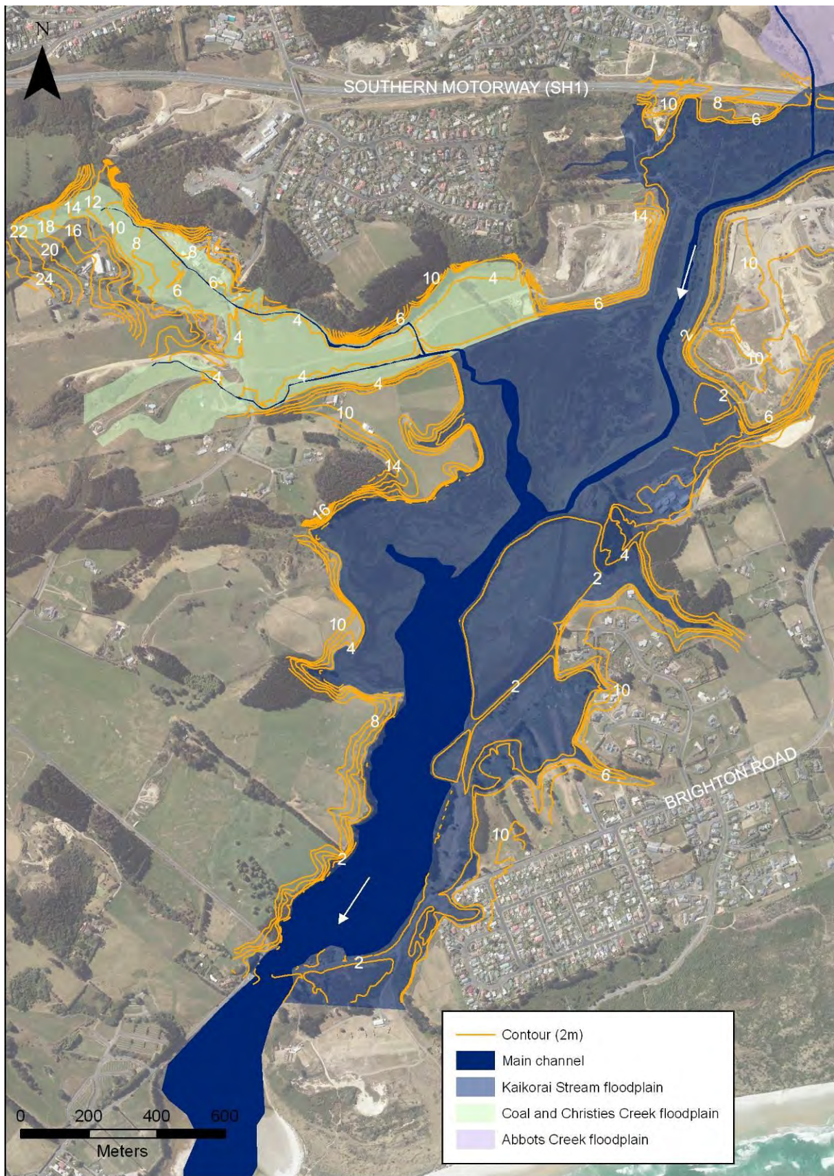
Figure 29 Kaikorai Stream, and Coal and Christies Creek floodplain area: Sunnyvale to the Brighton Road Bridge.
