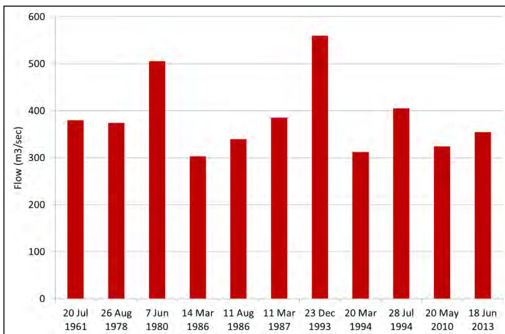
Figure 39 The 10 highest flows in the Taieri River at Sutton, since records commenced
