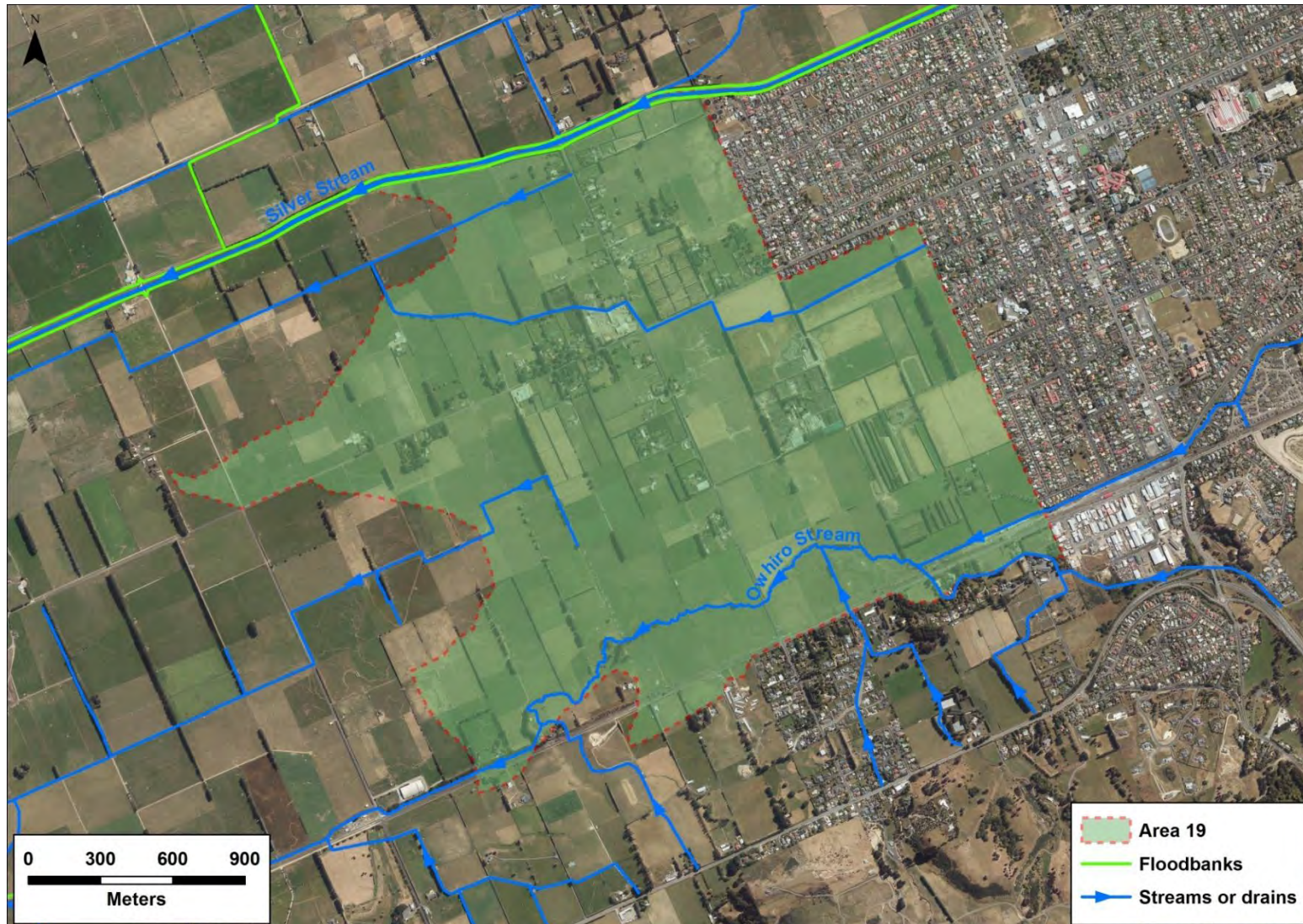
Figure 27 Area 19 – Streams and drains and general direction of flows in Area 19
