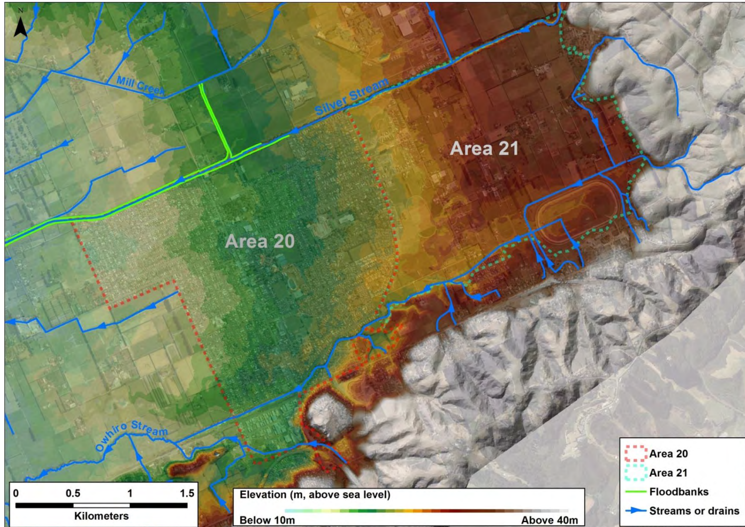
Figure 34 Topography of Area 20 and 21 (Mosgiel and Wingatui)
