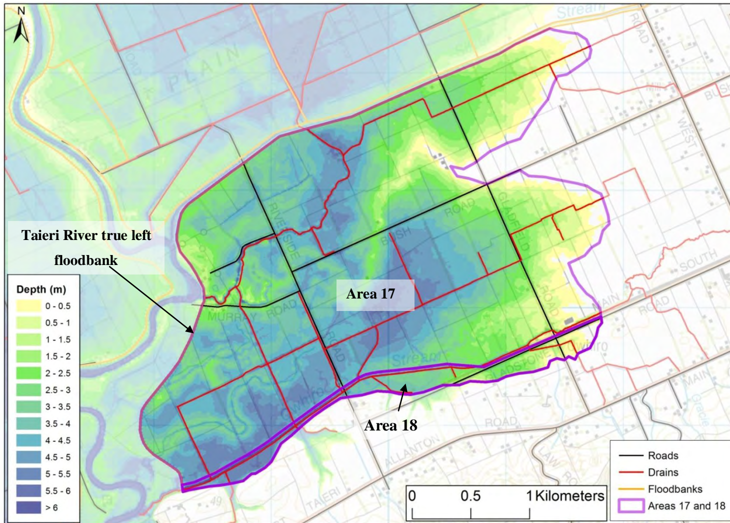
Figure 26 Depth of inundation in Area 17 and Area 18 if water was to reach the crest of the Taieri River true left floodbank
