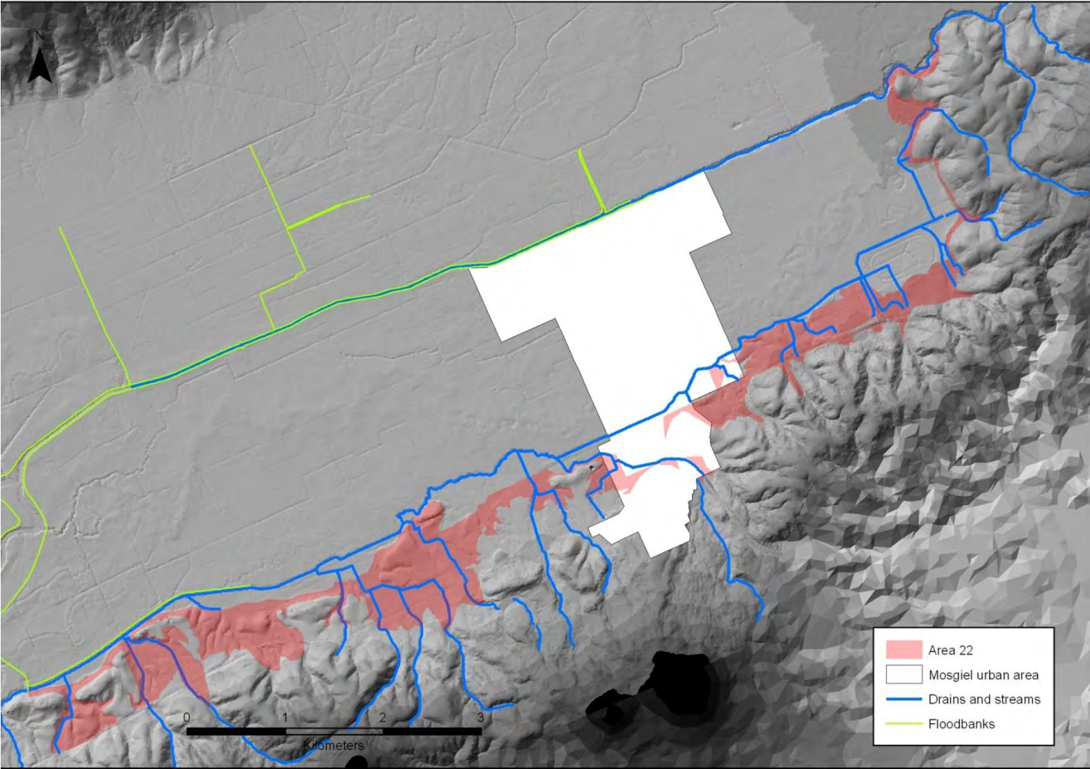
Figure 36 Coastal hill catchments which traverse Area 22
