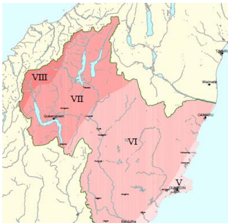
Figure 18. Map of Otago region showing MM Intensity expected to be exceeded once in 100 years (Murashev and Davey, 2005).
