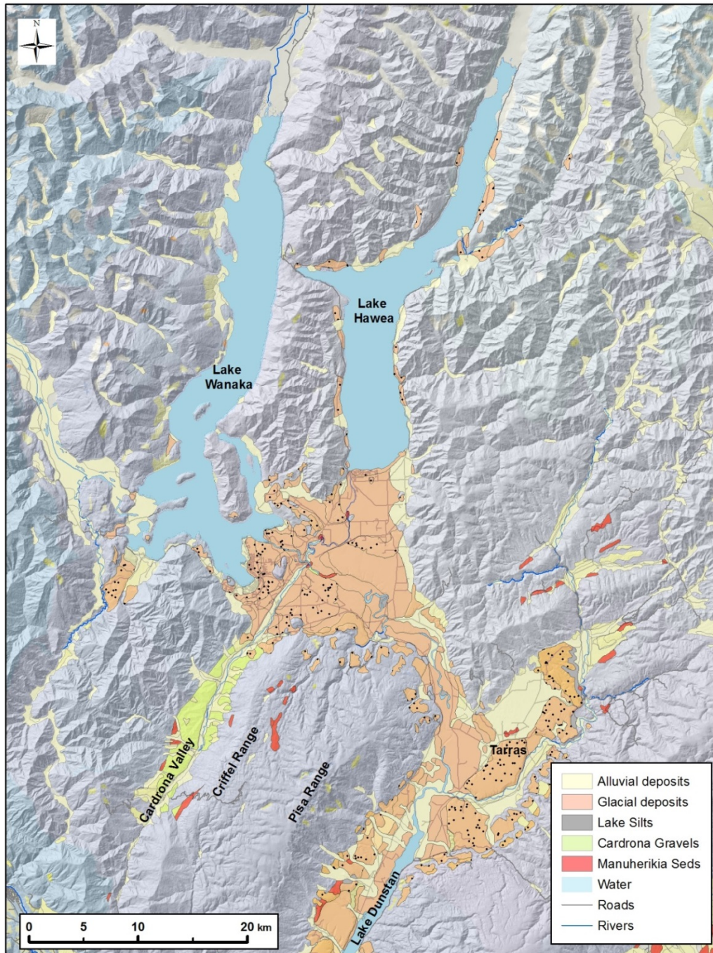
Figure 11. Geology of the Upper Clutha area. The pale blues and purples are varying metamorphic grades of schist bedrock. Glacial deposits (undifferentiated) and alluvial deposits occupy most of the valleys and lower hillslopes. Stippled areas represent glacial moraines. Remnants of Quaternary gravels persist in the Cardrona Valley, and isolated outcrops of the Tertiary Manuherikia sediments can be found southeast of Wanaka. Modified from QMAP (Turnbull, 2000).
