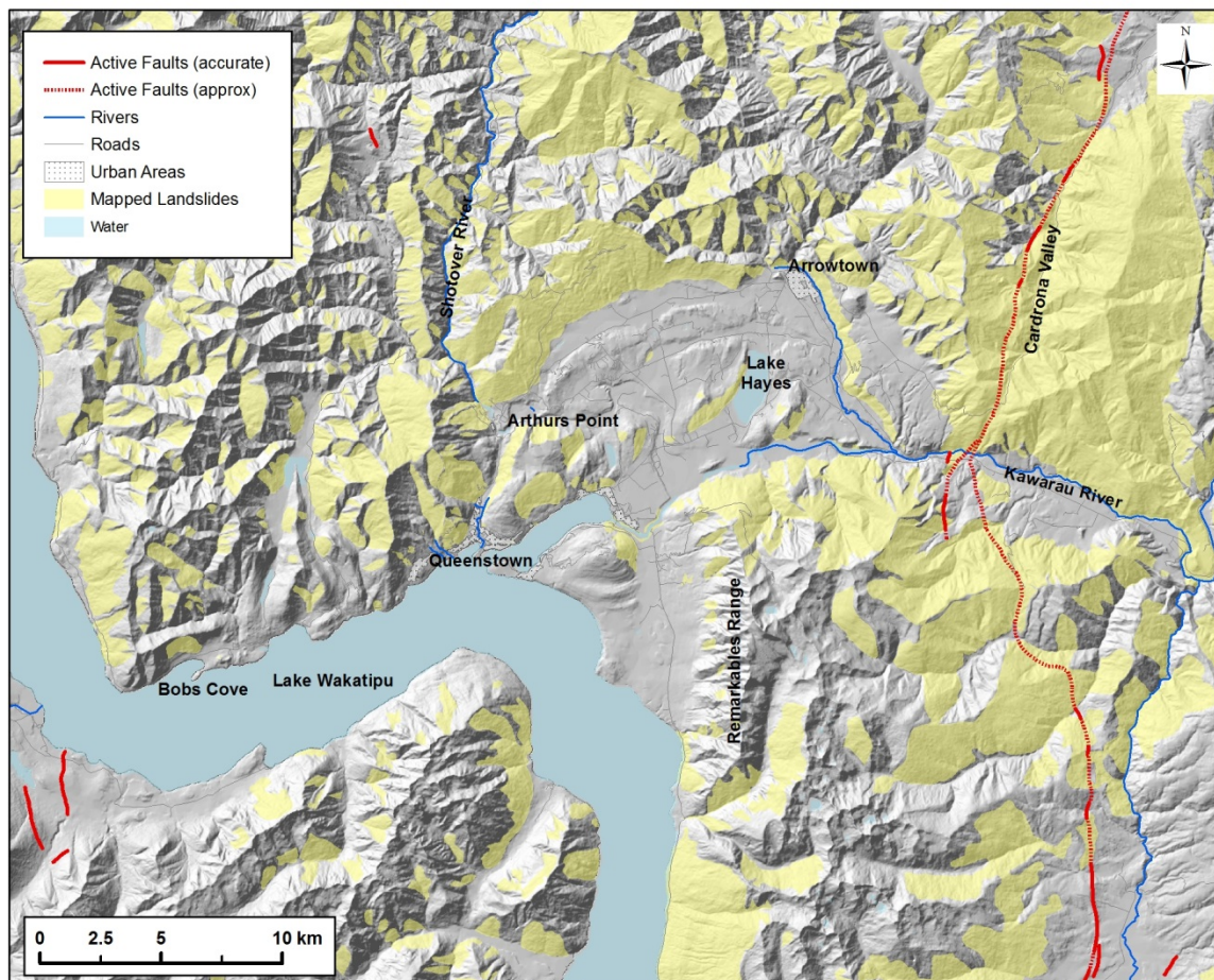
Figure 41. Mapped areas subject to mass movement hazards in the Wakatipu Area (ORC Natural Hazards Database).
