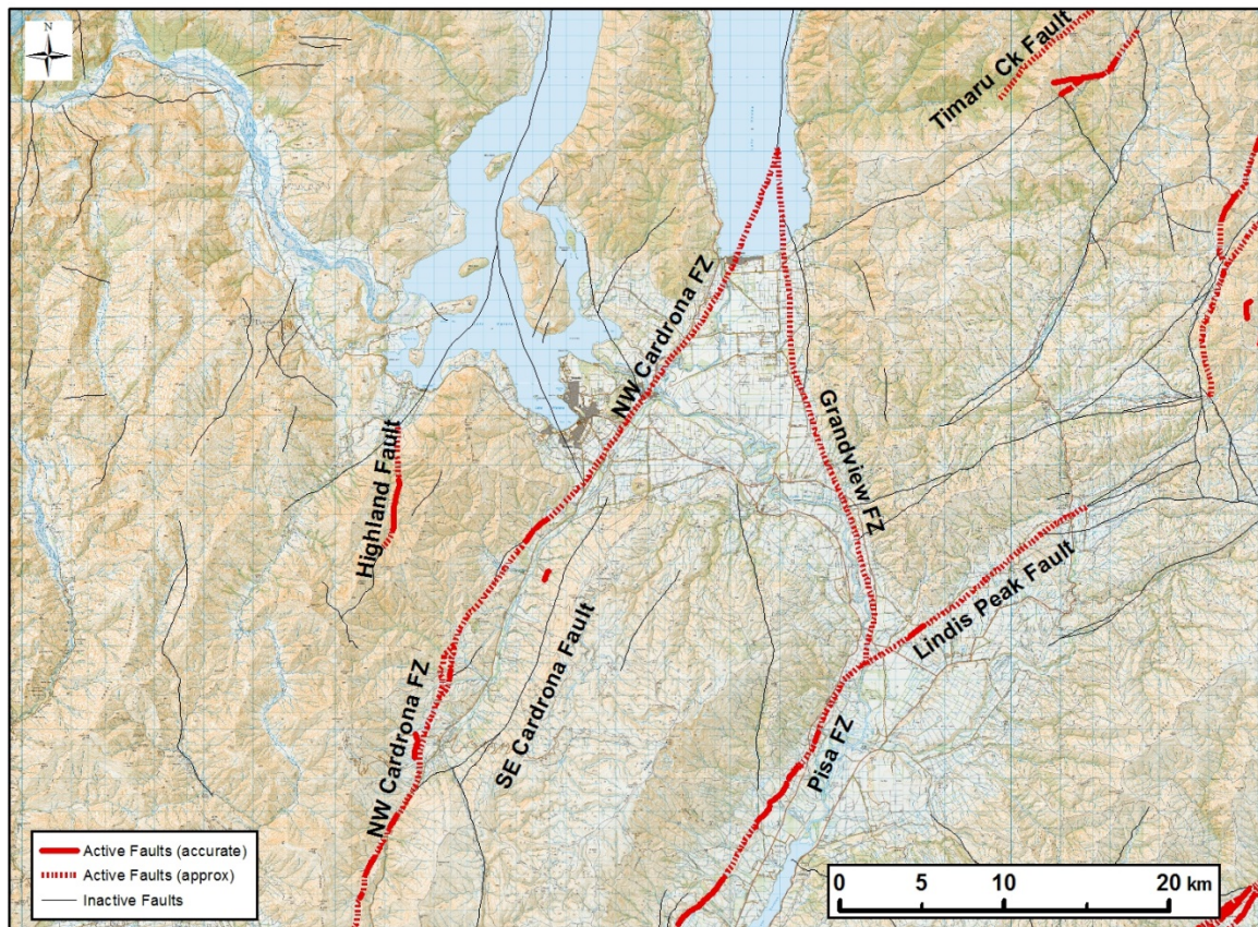
Figure 20. Active and inactive mapped faults near Wanaka. Active faults are mapped as either accurate (e.g., where there is a clear surface trace), or approximate. FZ = Fault Zone. From QMAP (Turnbull, 2000).
