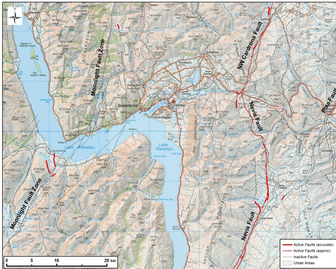
Figure 34. Topographic map of Wakatipu Area showing active and inactive faults. Modified from QMAP (Turnbull 2000).
