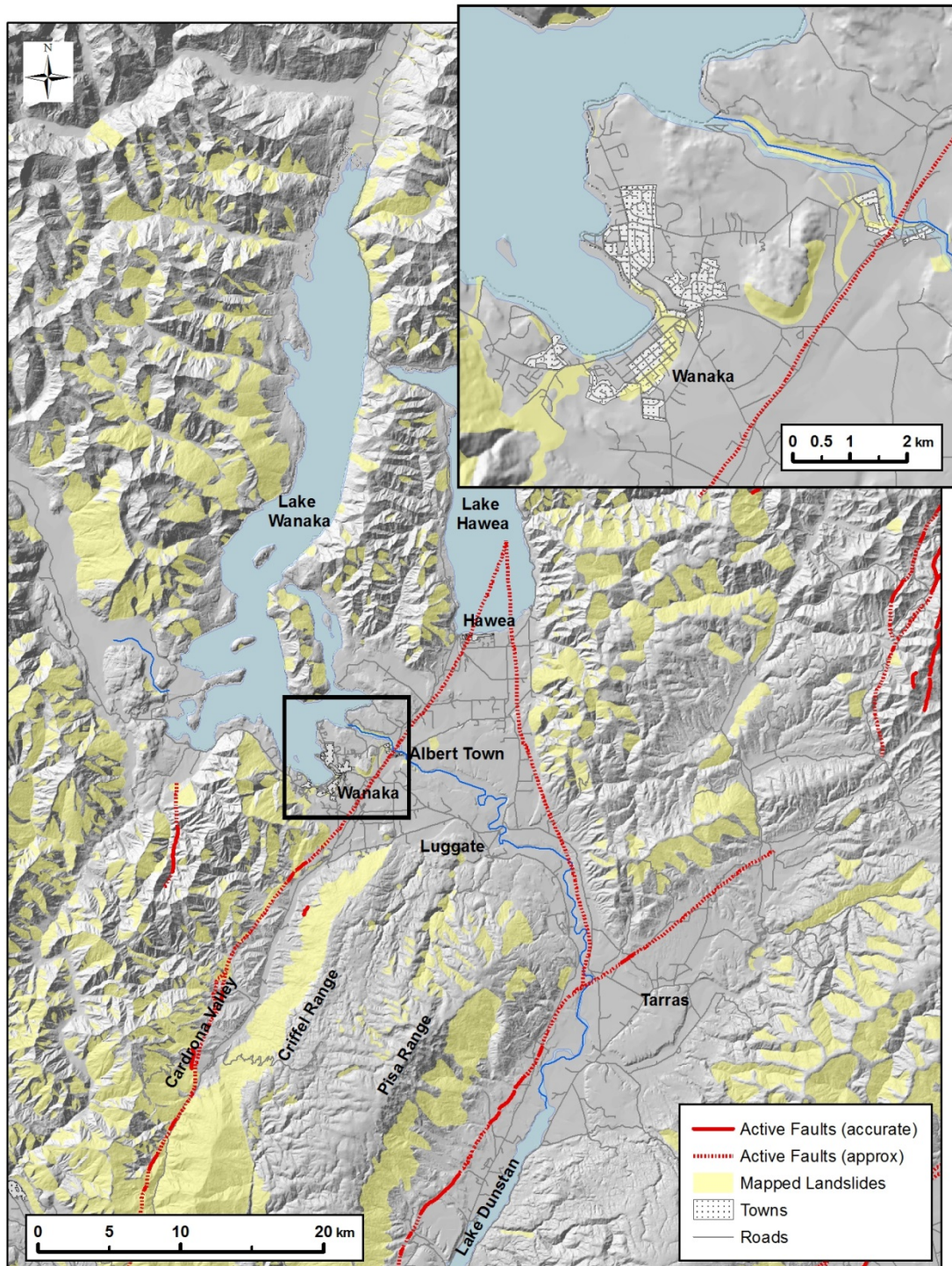
Figure 25. Mapped areas subject to mass-movement hazards in the Upper Clutha area (ORC Natural Hazard Database). Inset shows area around Wanaka Township.
