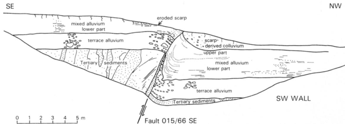
Figure 21. Diagram of a trench wall cut through active section of a splay of the Northern Cardrona Fault, just south of MacDonalds Creek (6 km north of Cardrona village). The ~18,000 year old alluvial terrace deposit (terrace alluvium layer) has been offset by 4 m vertically, by at least three recognised earthquakes (from Beanland and Barrow-Hurlbert, 1988)
