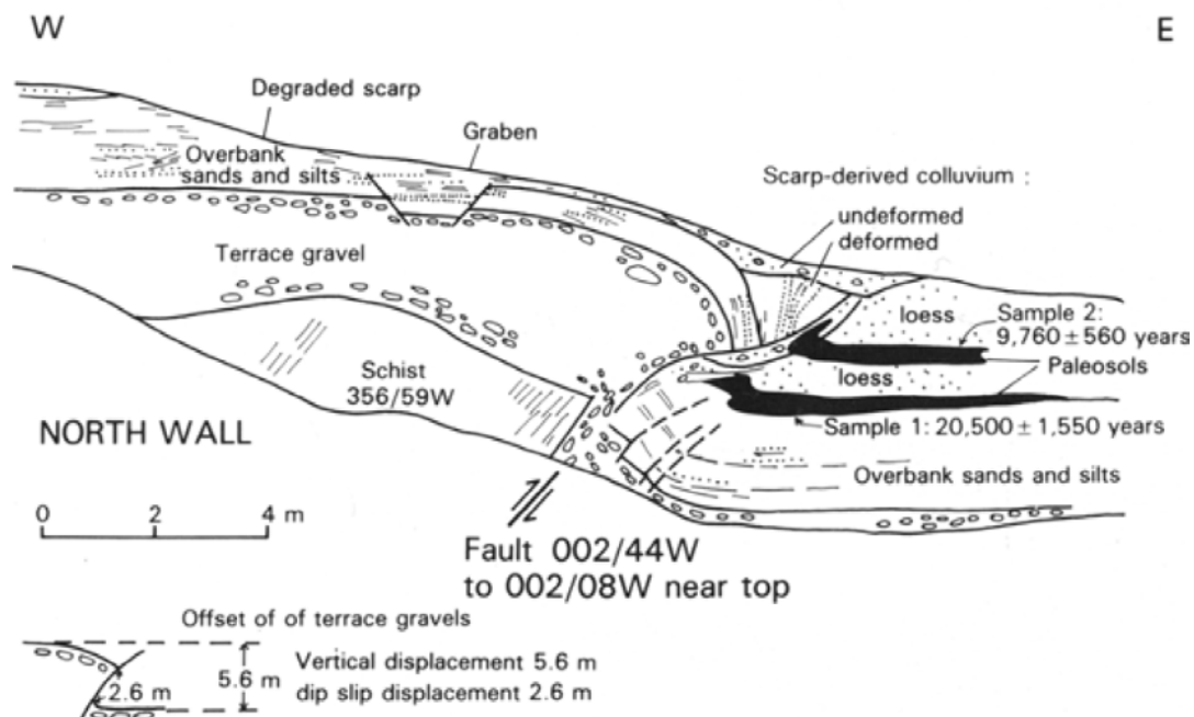
Figure 38. Cross section through the Kawarau Trace of the Nevis Fault on terrace above the Kawarau River. Evidence for three earthquakes can be seen in the deposits, which date to up to 23,000 years old (Beanland and Barrow Hurlbert, 1998).
