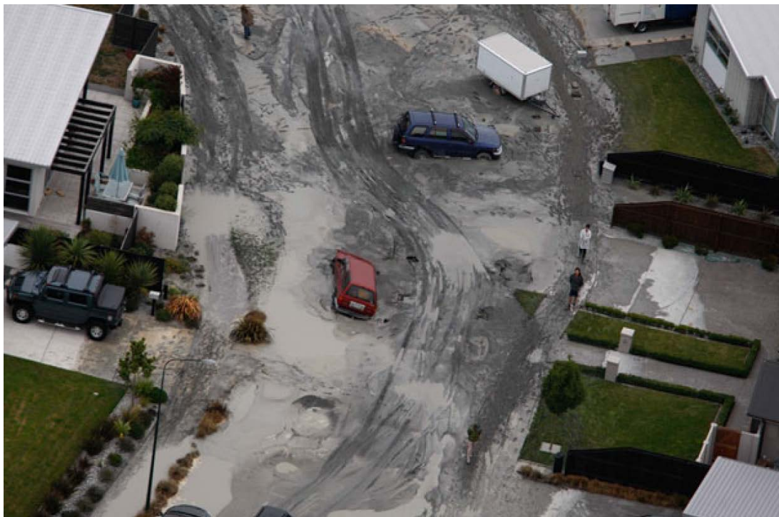
Figure 6. Liquefaction following the Christchurch 2011 Earthquake (Photo courtesy A. King, GNS Science)
