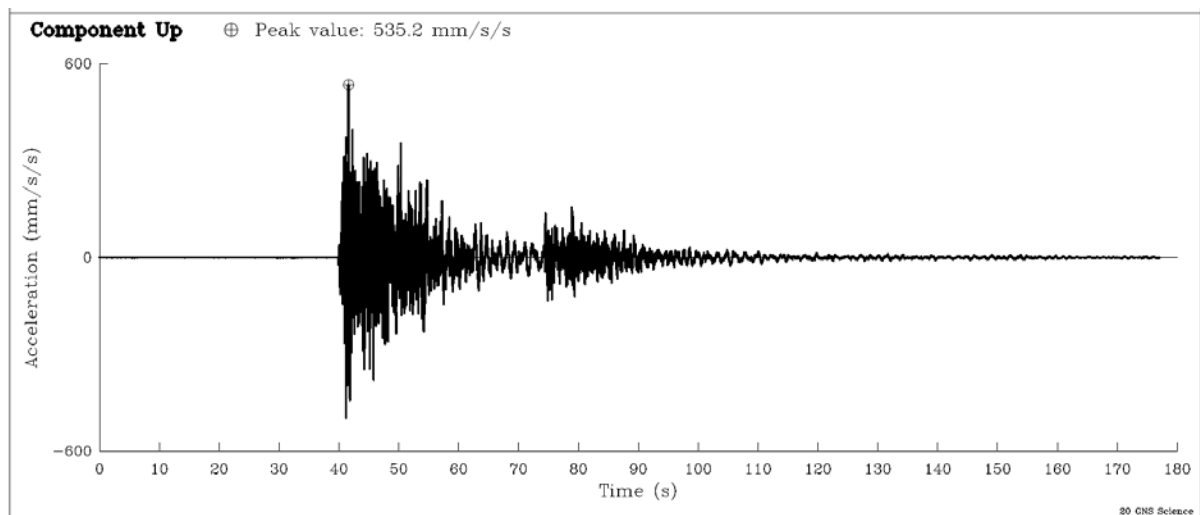
Figure 16. Seismograph record of vertical accelerations recorded at the Wanaka National Park headquarters during the May 4 th 2015 earthquake (Figure 17). This event caused some stock to fall from shop shelves in Wanaka, with a peak acceleration of 0.054 g (image from GNS Science.)
