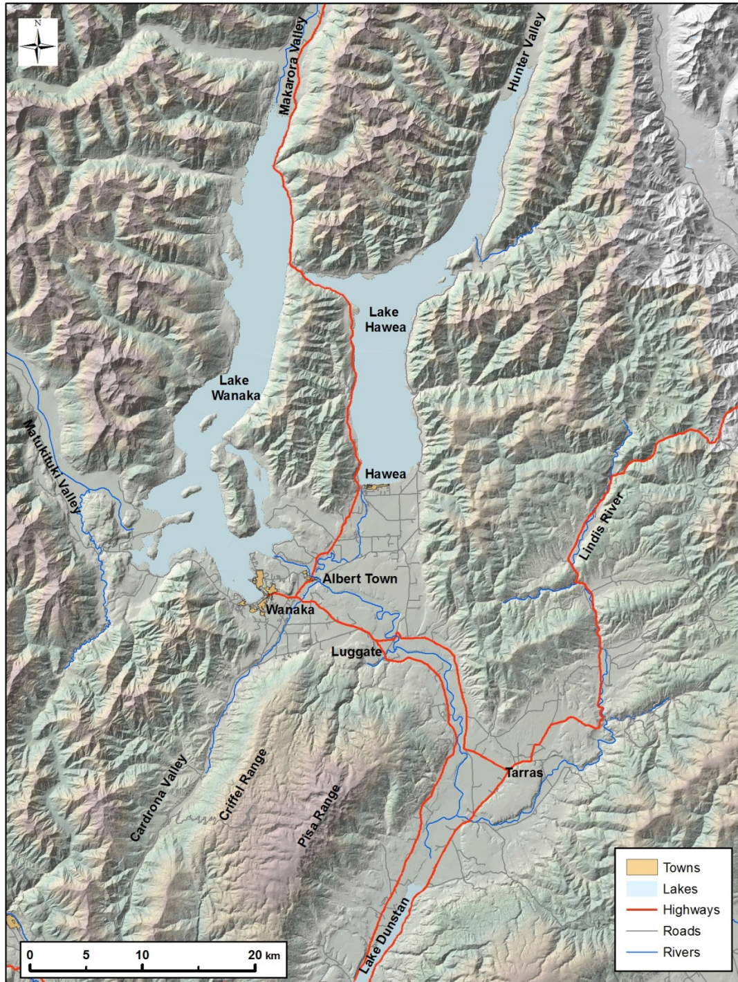
Figure 10. Upper Clutha study area and principal geographic features. The report focuses on the populated areas below the outlets of Lakes Wanaka and Hawea.
