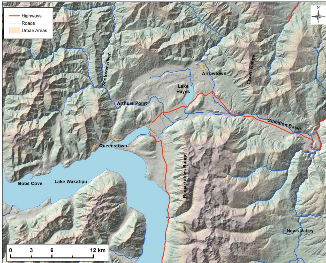
Figure 32. Wakatipu region study area and prominent geographic features. The report focuses on the populated areas surrounding Queenstown and Arrowtown, Bobs Cove, and the Kawarau Gorge down to the Gibbston Basin.
