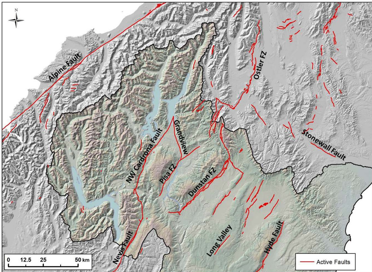
Figure 12: Active faults in west Otago and surrounding regions (From QMAP and GNS Active Fault Database). Otago region is outlined.
