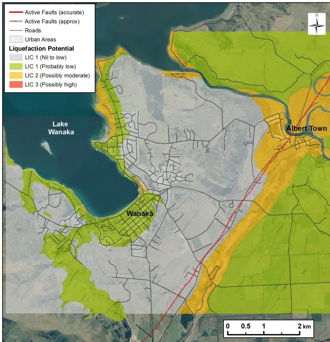
Figure 24. Map of liquefaction risk in the Wanaka area assessed by Tonkin & Taylor Ltd (2012) for the Queenstown Lakes District Council. The most susceptible layers are river courses and some lake margin areas. The mapping is intended to guide the appropriate level of site investigation at the development stage, rather than assess the likelihood of liquefaction at a site.
