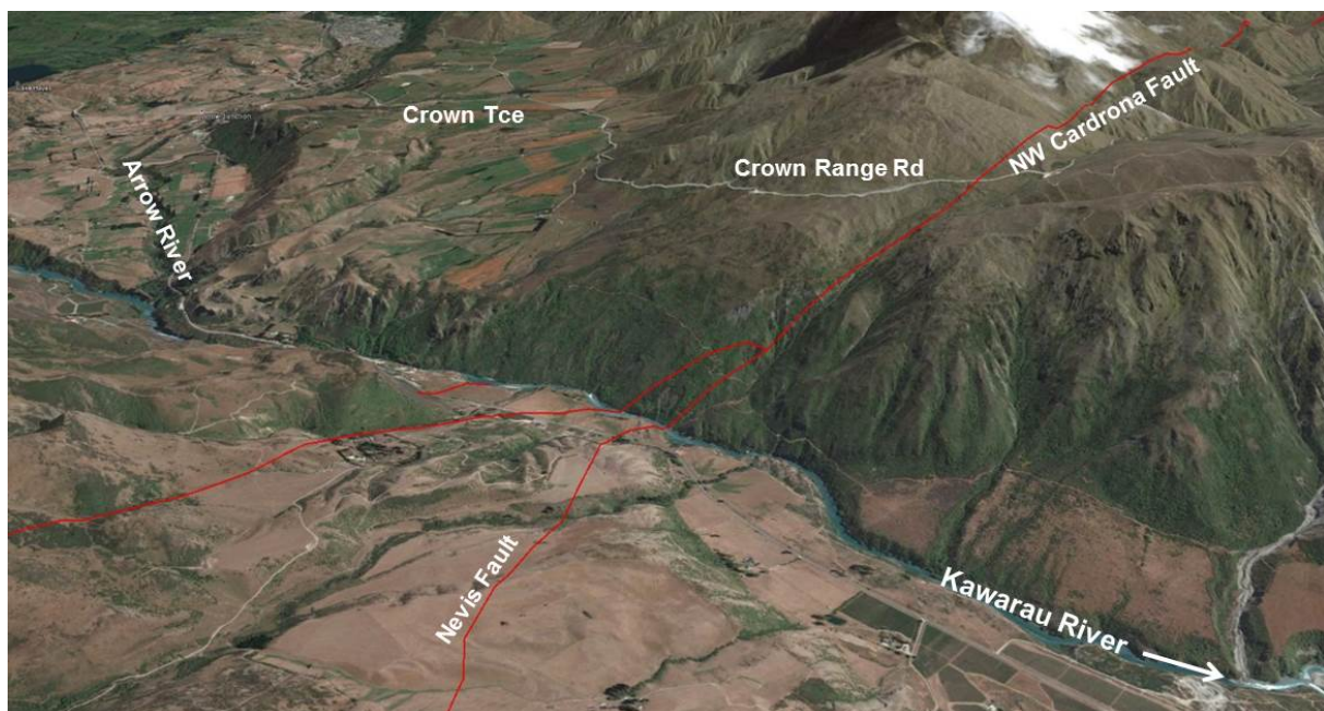
Figure 37. Oblique view of the upper Kawarau Gorge towards the Northwest. The Nevis Cardrona Fault (red) runs across the gorge and continues along the Cardrona Valley. The trench in Figure 38 is across the upstream-most strand (Kawarau Trace). The Fault runs through a large landslide complex on the north side of the valley. The Crown Range Road can be seen climbing up from the Crown Terrace and crossing the fault near the summit (Google Earth).
