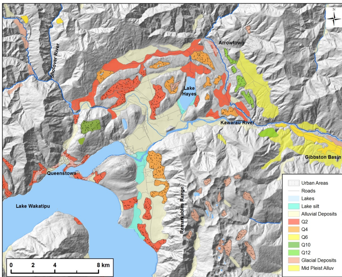
Figure 35. Glacial deposits in the Wakatipu area. 'Q' denotes glacial age based on Oxygen isotope stage (See Appendix C). Modified from QMAP (Turnbull, 2000)
