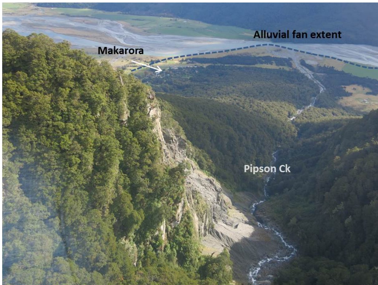
Figure 30. View down Pipson Creek near Makarora (May 2015). The eroding cliffs in the foreground (and other cliffs upstream) contribute rock and sediment to the channel, which can mobilise into debris flows during high rainfall. Earthquake shaking is liable to cause extensive rockfall and landsliding into the creek.
