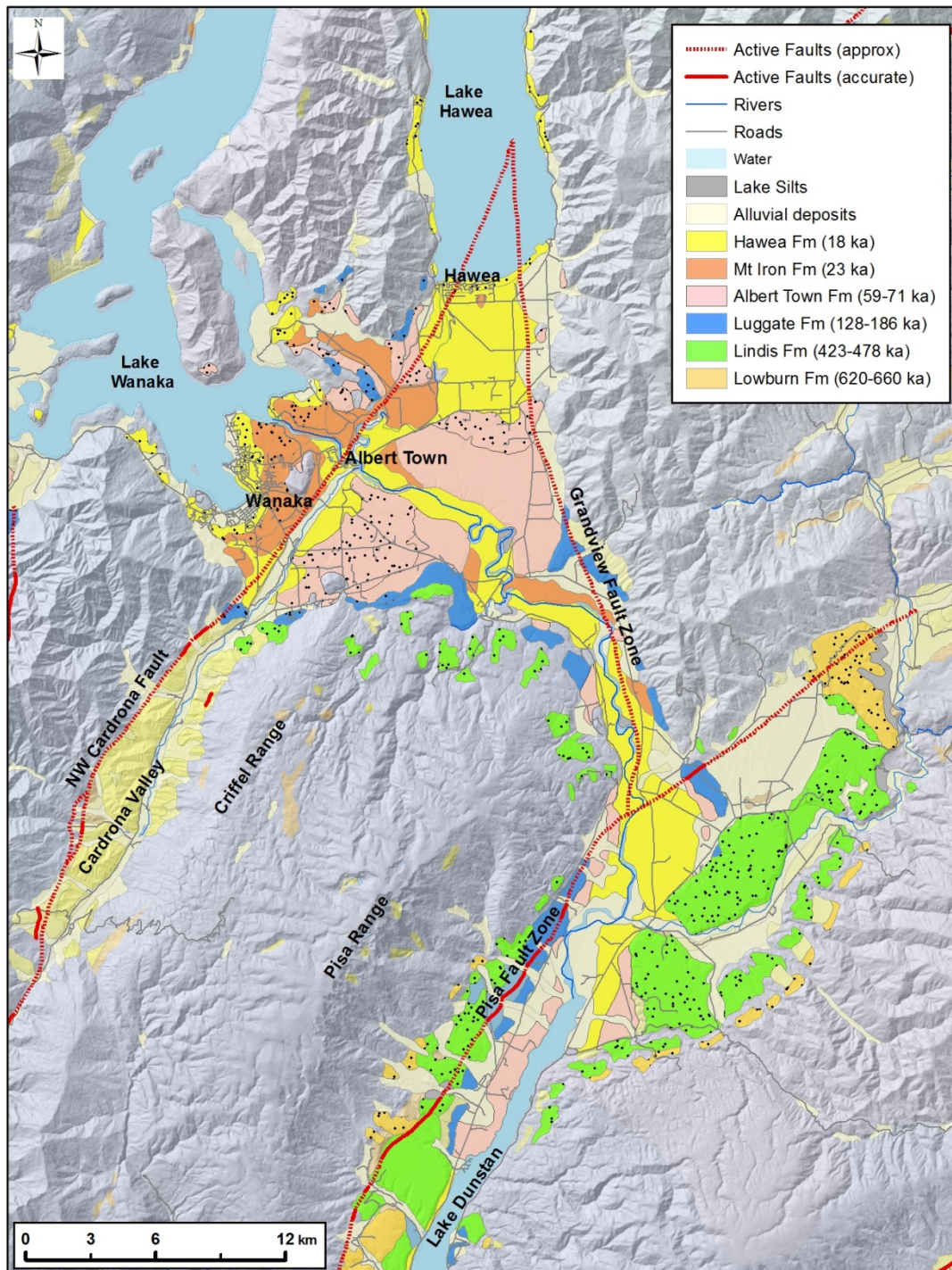
Figure 48. Glacial advances in the Upper Clutha area. Each advance has a moraine (stippled) and an associated outwash plain. Modified from QMAP (Turnbull, 2000).
