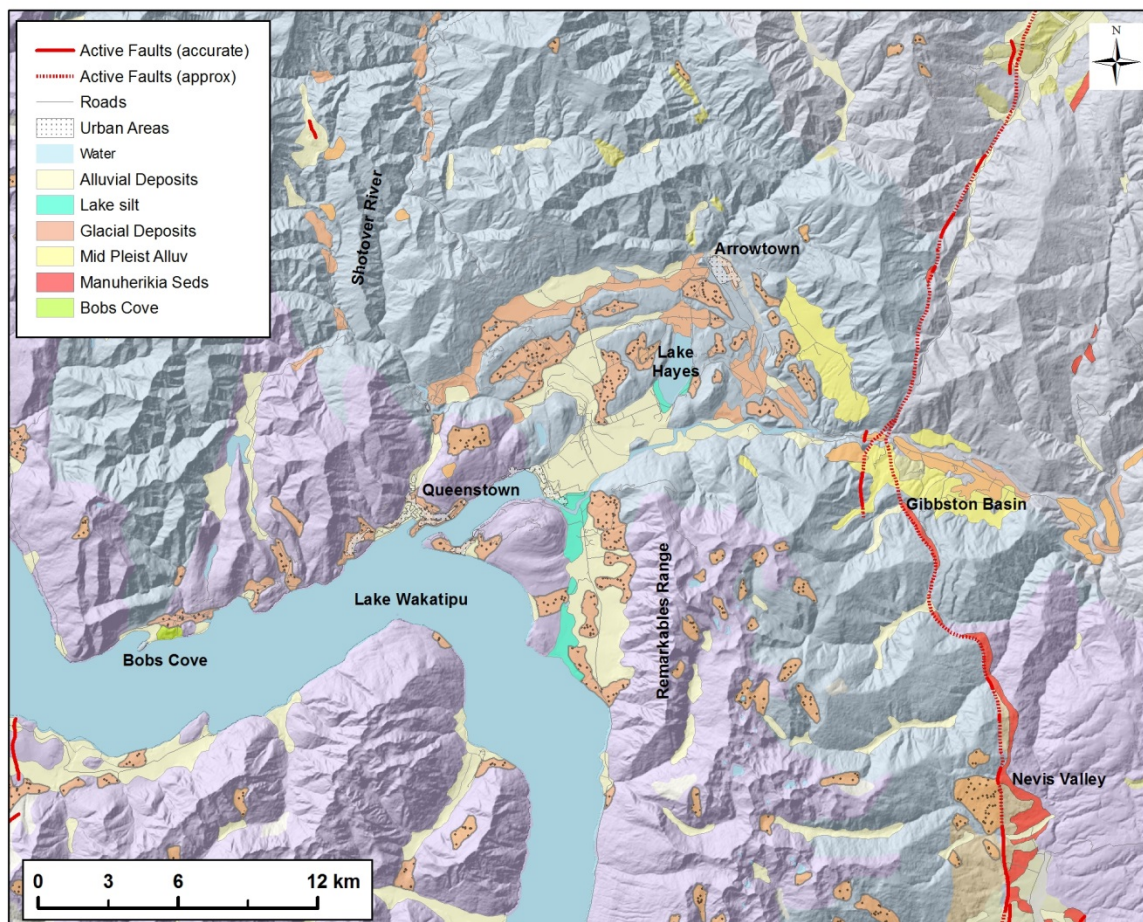
Figure 33. Geology of the Wakatipu area. The pale blues and purples are varying metamorphic grades of schist bedrock. Glacial deposits (undifferentiated) and alluvial deposits occupy most of the valleys and lower hillslopes. Lake silts were deposited during a higher lake level. Isolated outcrops of the Tertiary Manuherikia sediments can be found east of the Nevis Cardrona Fault zone. Modified from QMAP (Turnbull, 2000).
