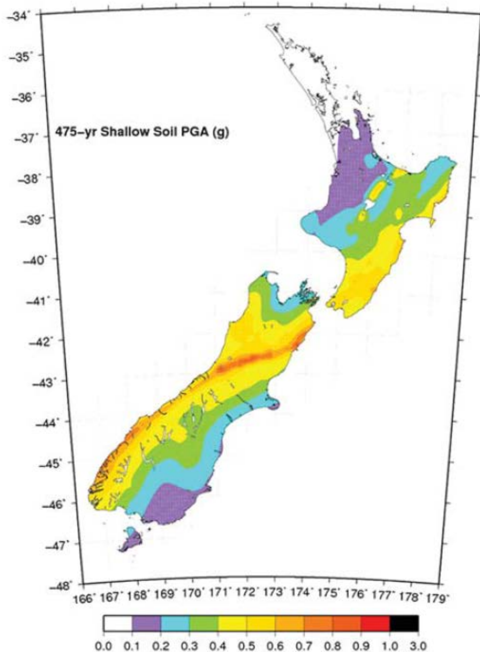
Figure 19. Probabilistic seismic hazard map for New Zealand (Stirling et al. 2012). This map shows the maximum expected peak ground acceleration (relative to gravity) expected over a 475 year period. The zone of red down the west of the South Island follows the Alpine Fault.
