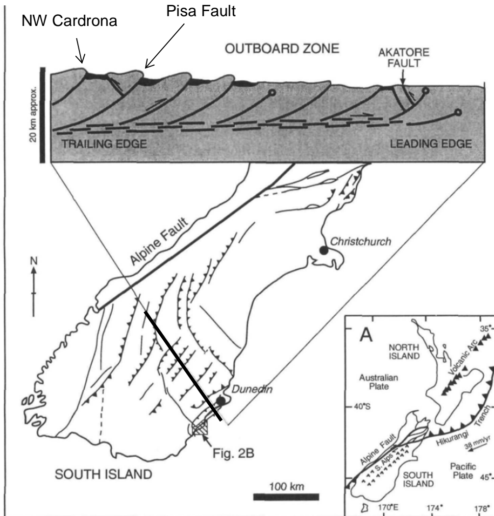
Figure 47. Major faults form a series of tilted blocks across the Otago region. The NW Cardrona Fault and Pisa fault are the western-most faults. (From Litchfield and Norris, 2000).
