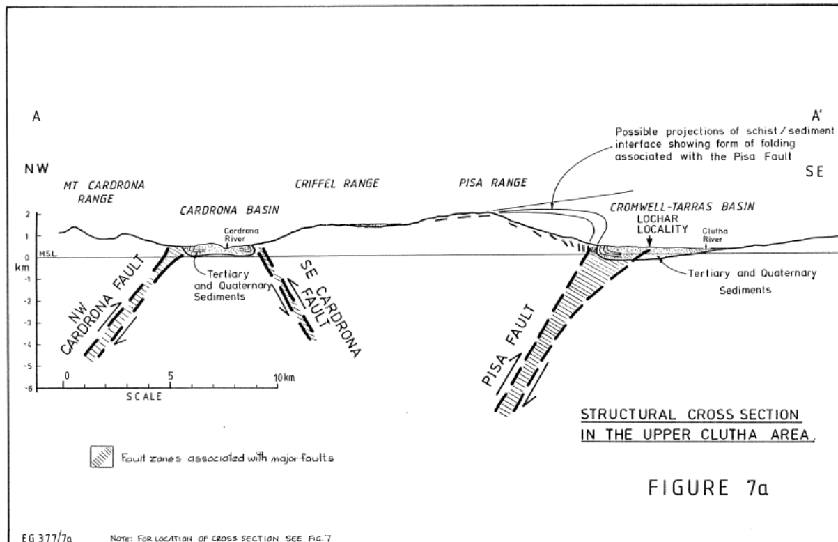
Figure 15. NW-SE oriented cross-section through the Cardrona Valley and Cromwell Basin (marked on Figure 14) showing the orientation of major fault structures (Officers, 1984). Tertiary sediments remain preserved along the valley floors, but have been removed by erosion at higher elevations.
