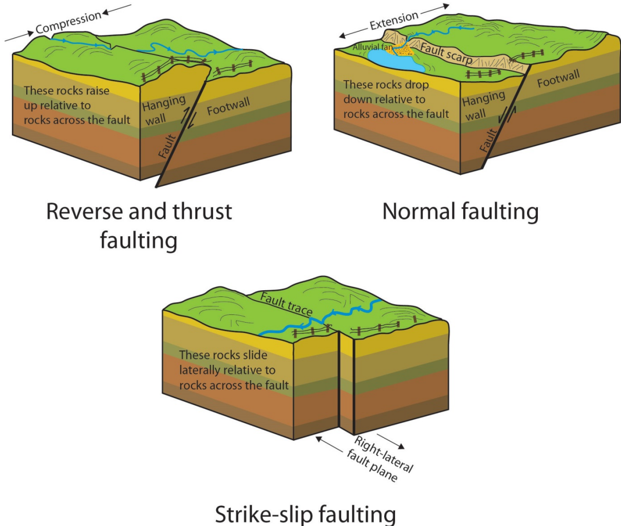
Figure 2. The main styles of faulting. Faults in western Otago are primarily Reverse Faults, reflecting the regional compression, whereas the Alpine Fault is a predominantly a strike-slip fault (From USDA National Park Service).
