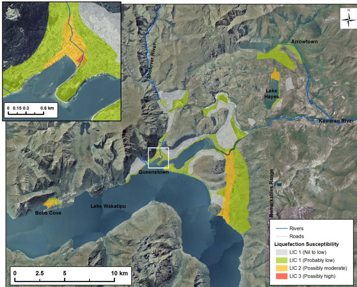
Figure 40. Map of liquefaction risk in the Wakatipu Region assessed by Tonkin & Taylor Ltd (2012) for the Queenstown Lakes District Council. The most susceptible layers are river courses and lake margin areas, particularly areas underlain by lake silts. Inset shows downtown Queenstown area. The mapping is intended to guide the appropriate level of site investigation, rather than assess the likelihood of liquefaction at a site.
