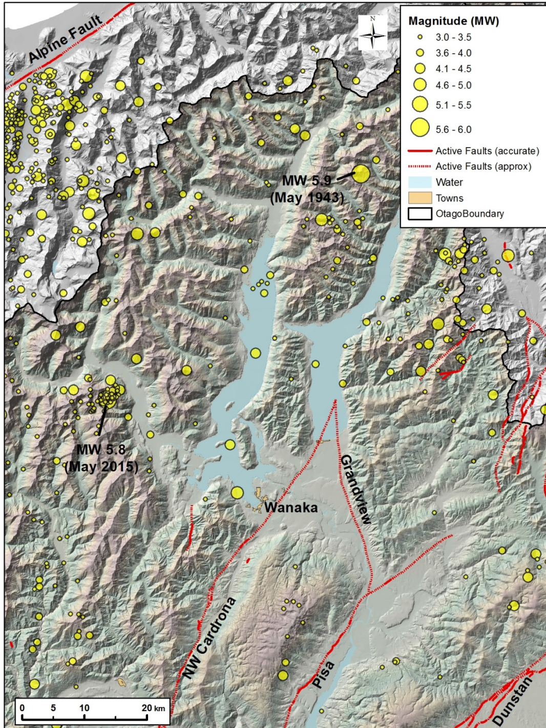
Figure 17. Historic seismicity in the west Otago area, with earthquakes larger than M_w 3.0 from 1942 – July 2015. Two earthquakes larger than M_w 5.5 have been recorded over that period. The highest concentration of earthquakes occurs towards the Alpine Fault in the northwest of the mapped area. Data from GeoNet (accessed July 2015).
