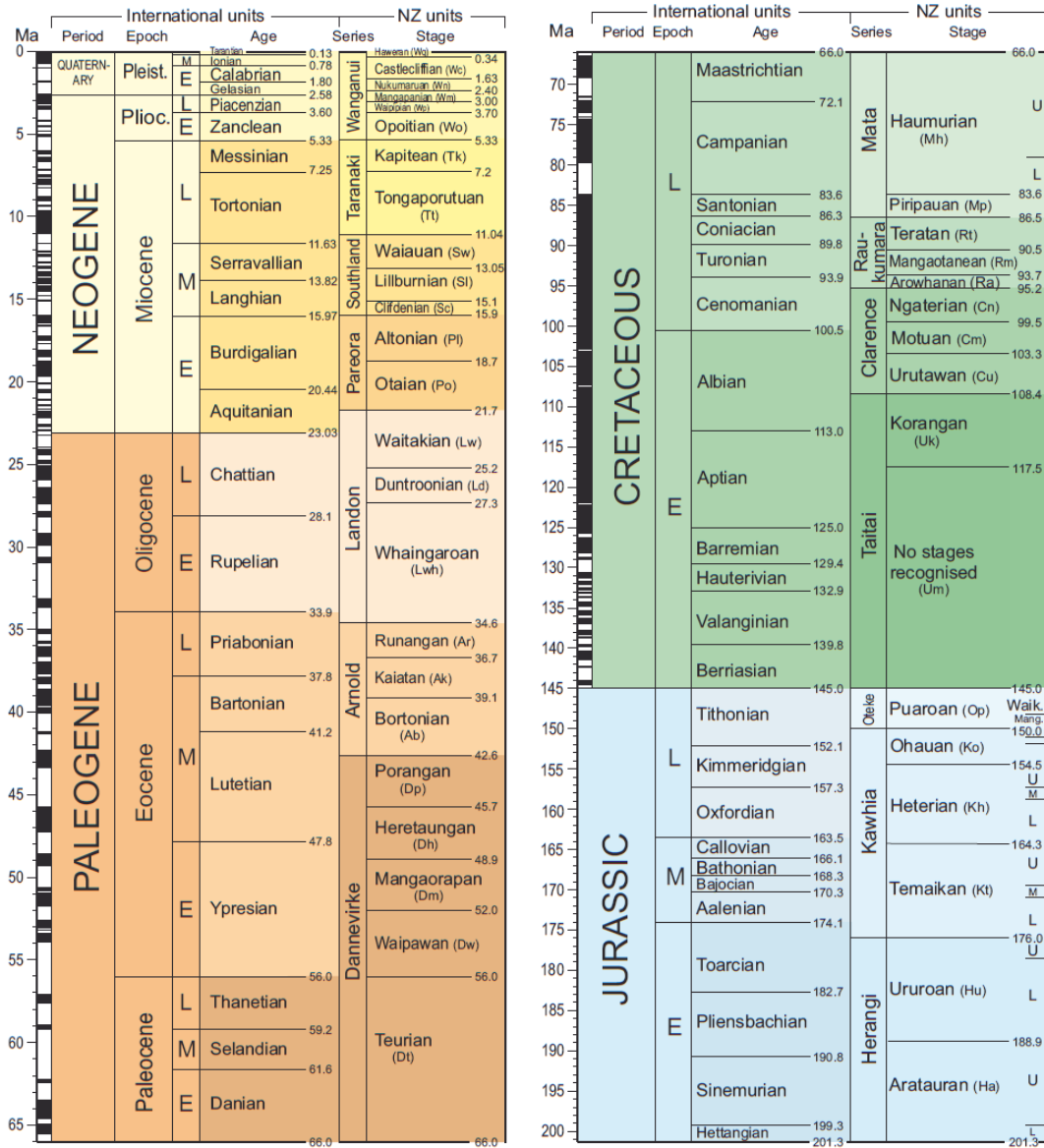
Geologic time scale (Jurassic-Present). From GNS Science.
