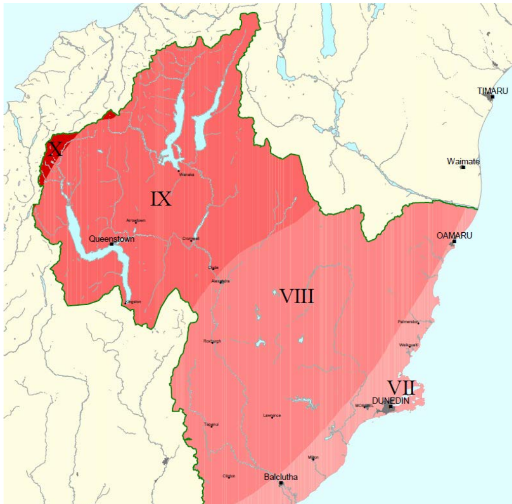
Figure 39. Map of Otago region showing MM Intensity expected to be Exceeded once in 2500 years (Murashev and Davey, 2005). See also Figure 18 for 100 year exceedence map.
