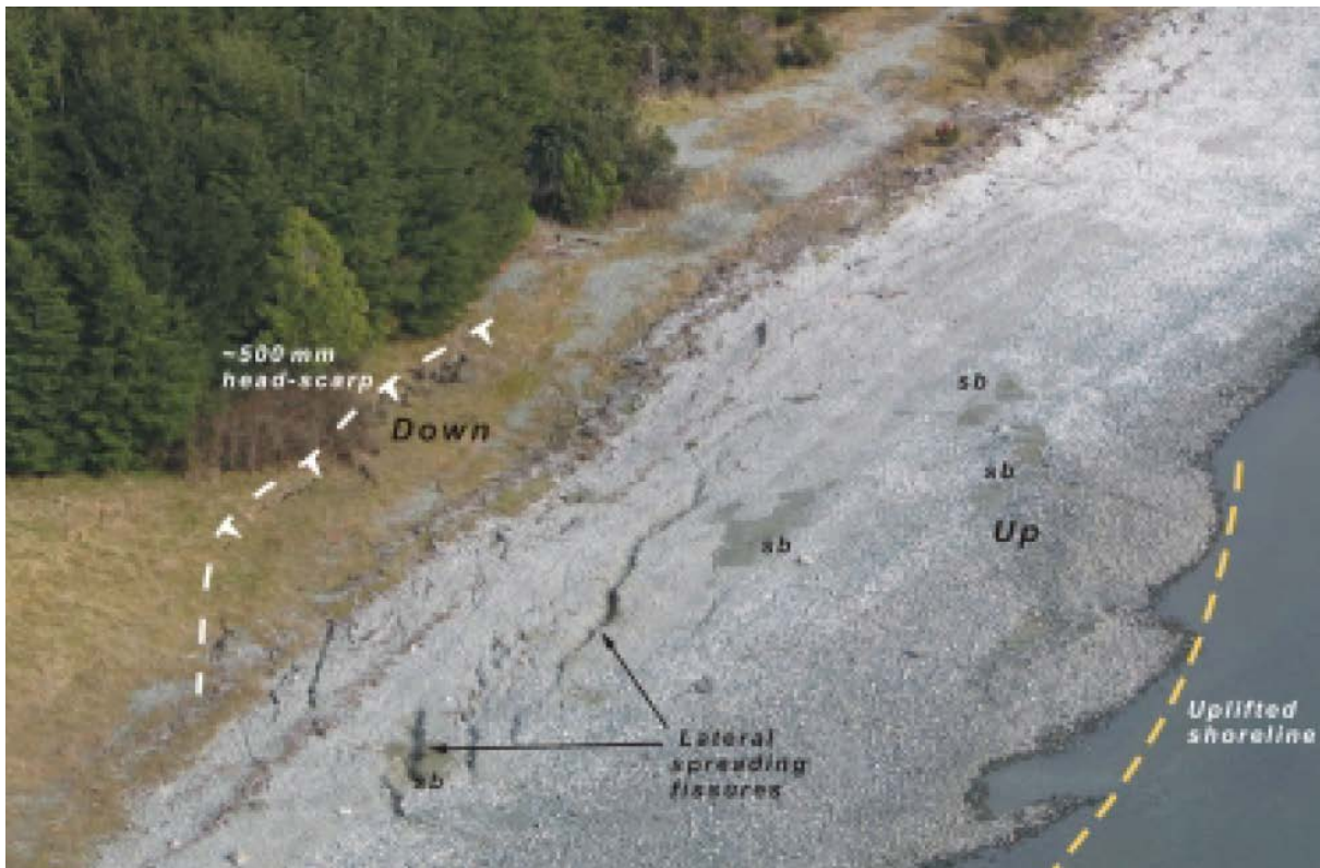
Figure 7. Lake edge failure along Lake Te Anau during the 2003 Fiordland earthquake (Hancox et al. 2003). This failure incorporated liquefaction and lateral spreading of the lake beach area.
