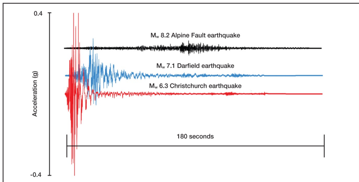
Figure 3. Seismographs from two Canterbury Earthquakes as recorded in Christchurch in Sept 2010 (blue line) and Feb 2011 (red line). The Black line is a synthetic seismograph predicting the level and duration of shaking recorded in Christchurch during a hypothetical Alpine Fault earthquake. The more distant but larger Alpine Fault event has less intense ground shaking, but continues for a much longer duration (Webb et al., 2011).
