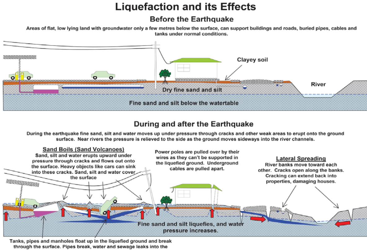
Figure 5. Effects of liquefaction (from IPENZ Factsheet)
