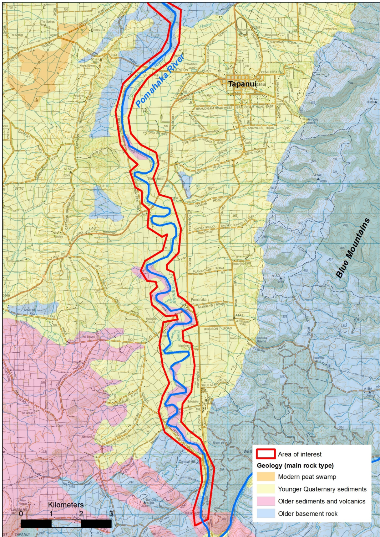
Figure 5. Geological map showing the reach of the Pomahaka between the Kelso Gorge to Conical Hill
