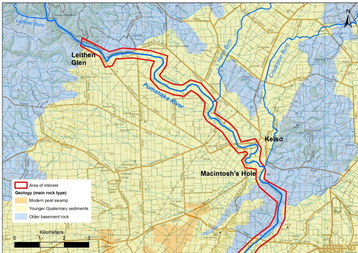
Figure 4. Geological map showing the reach of the Pomahaka River between Dusky Forest and the Kelso Gorge
