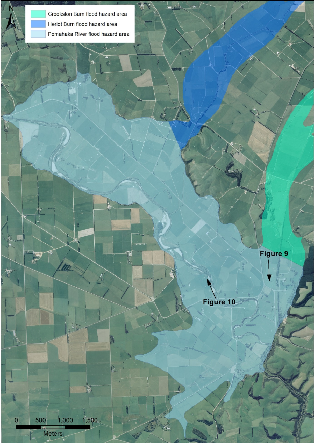
Figure 11. Pomahaka flood hazard area extent (Kelso floodplain) (ORC, 1999)
