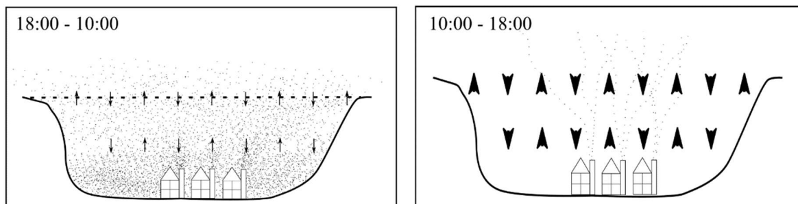
Fig. 1.8. A schematic of the typical inversion and PM10 characteristics in Alexandra. Night time radiative cooling decreases the mixing between the SBL and RL, which leads to high PM10 concentrations in the SBL. During the day, radiative warming at the surface increases the dispersion of PM10, reducing PM10 concentrations in the SBL.
