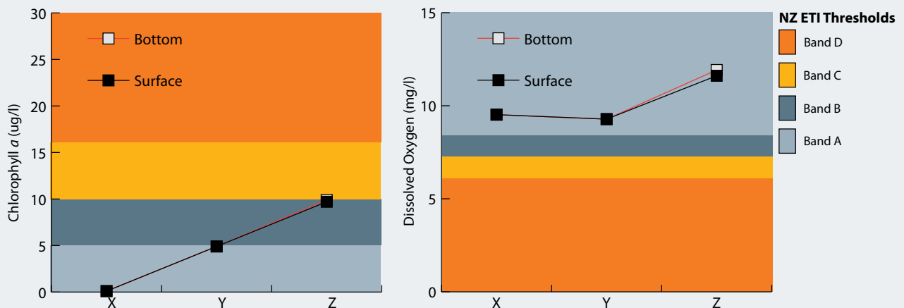
Figure 15. Chlorophyll a and dissolved oxygen concentrations in surface and bottom water, Catlins Estuary, 17 December 2016.
