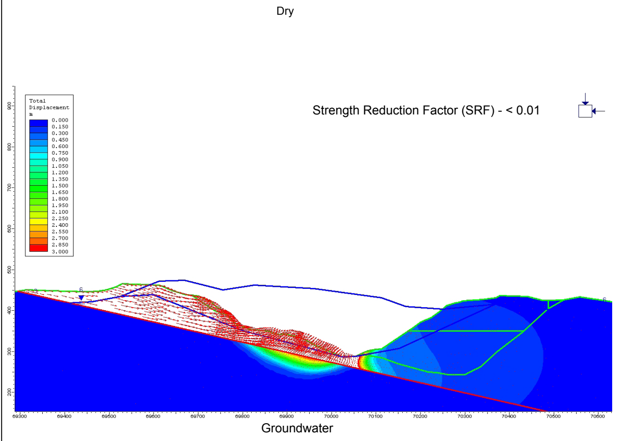
Oceana Gold Round Hill East ANALYSIS OF ROUND HILL PIT STABILITY 1998 MINING TOTAL DISPLACEMENT PSM 71-107R Figure C3
