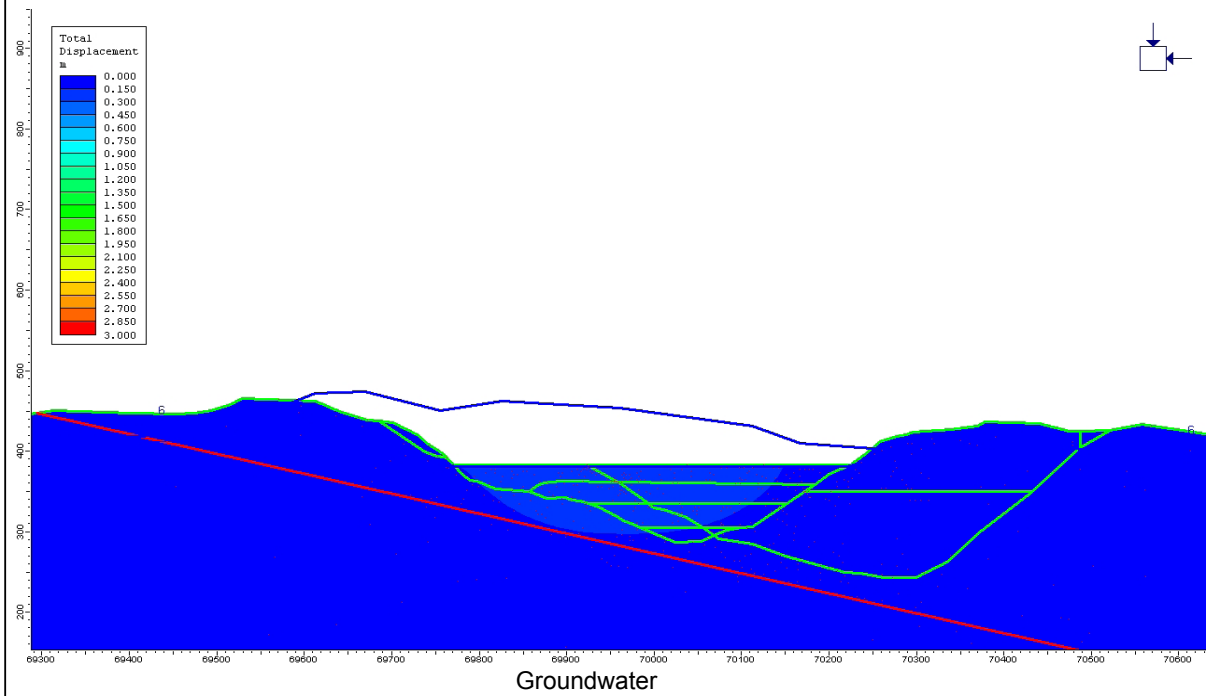
Oceana Gold Round Hill East ANALYSIS OF ROUND HILL PIT STABILITY 1996 MINING TOTAL DISPLACEMENT PSM 71-107R Figure C2
