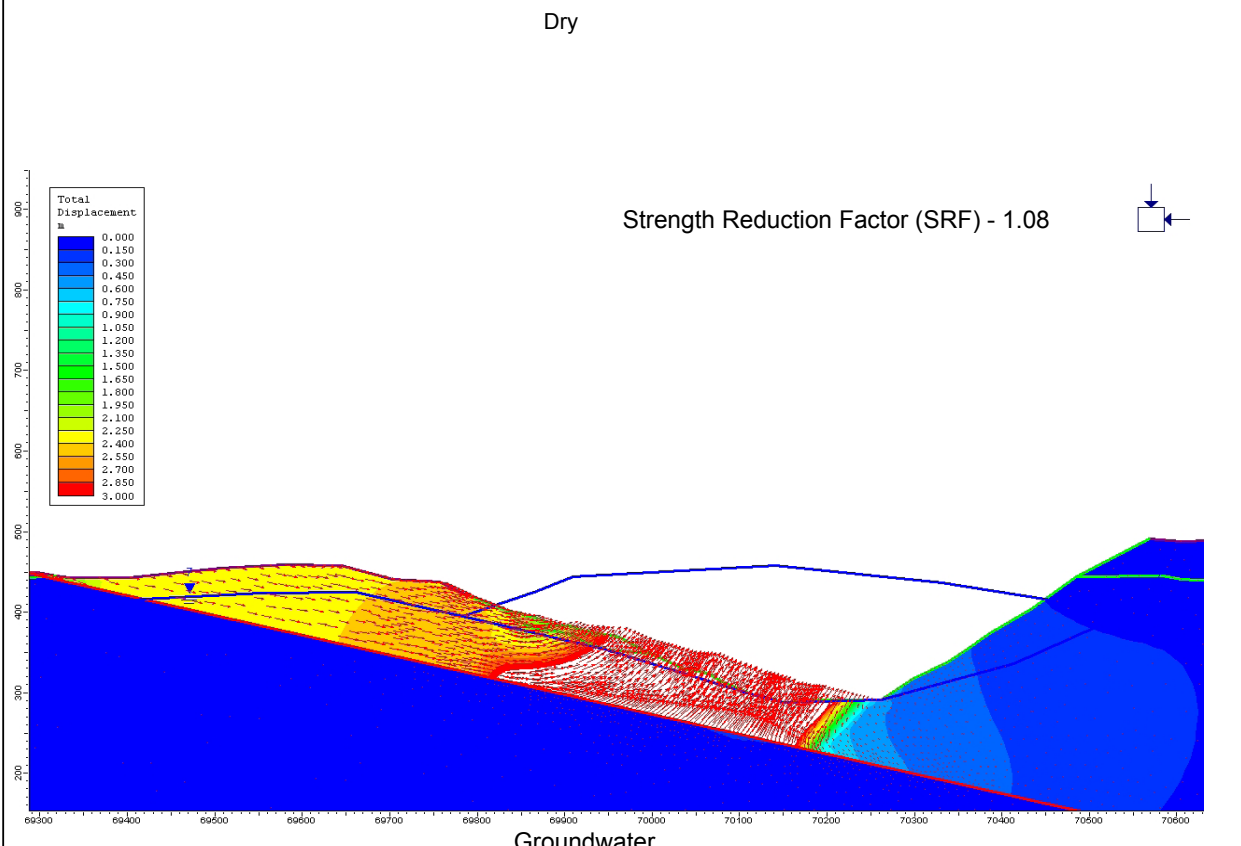
Oceana Gold Round Hill East ANALYSIS OF ROUND HILL PIT STABILITY PROPOSED MINING STAGE 2 TOTAL DISPLACEMENT PSM 71-107R Figure C8
