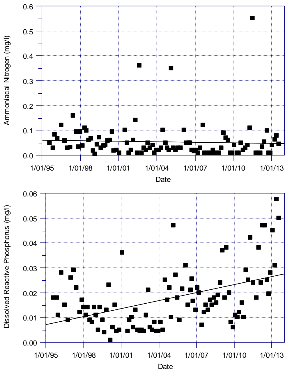
Figure 10 \text{NH}_4\text{-N} and DRP trends in Lake Tuakitoto at the outlet (1995 to 2013)
