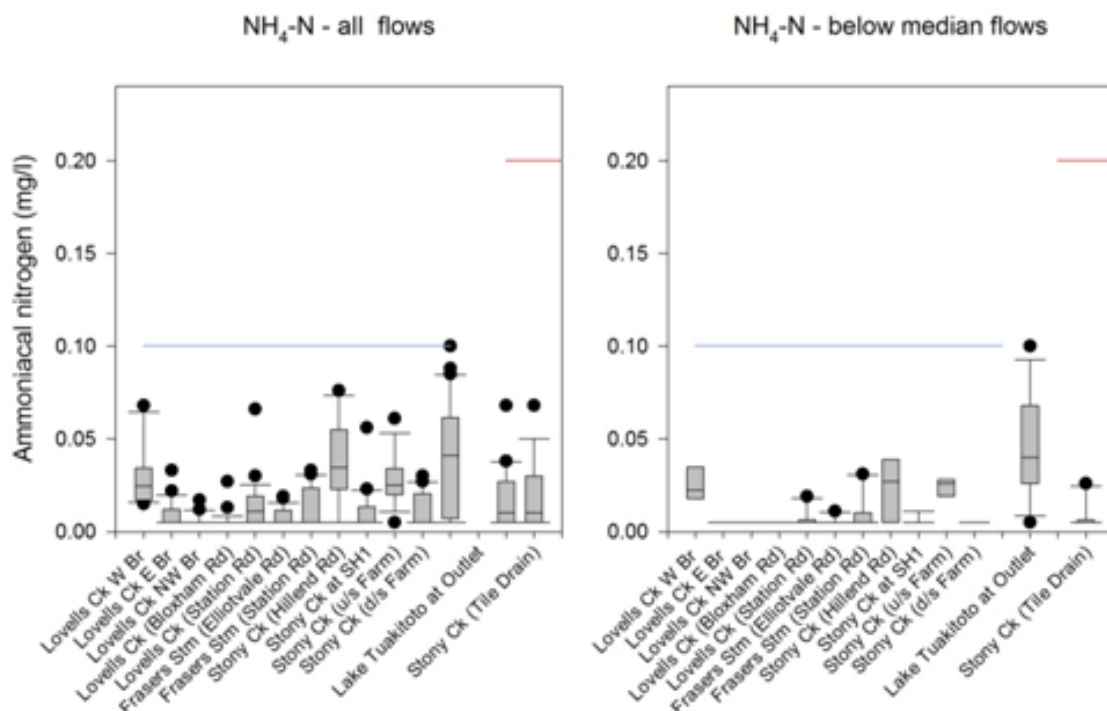
Figure 18 Ammoniacal nitrogen concentrations in the Lake Tuakitoto catchment. Plan Change 6A Schedule 15 limits are represented by the blue line (Group 1) and the red line (Group 4)
