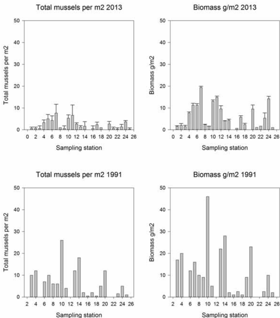
Figure 23 Comparison of 1991 (Ogilvie, 1995) and 2013 (ORC) data for the density (no/m 2 ) and biomass (g/m 2 AFDW) of mussels at 25 sampling stations in Lake Tuakitoto
