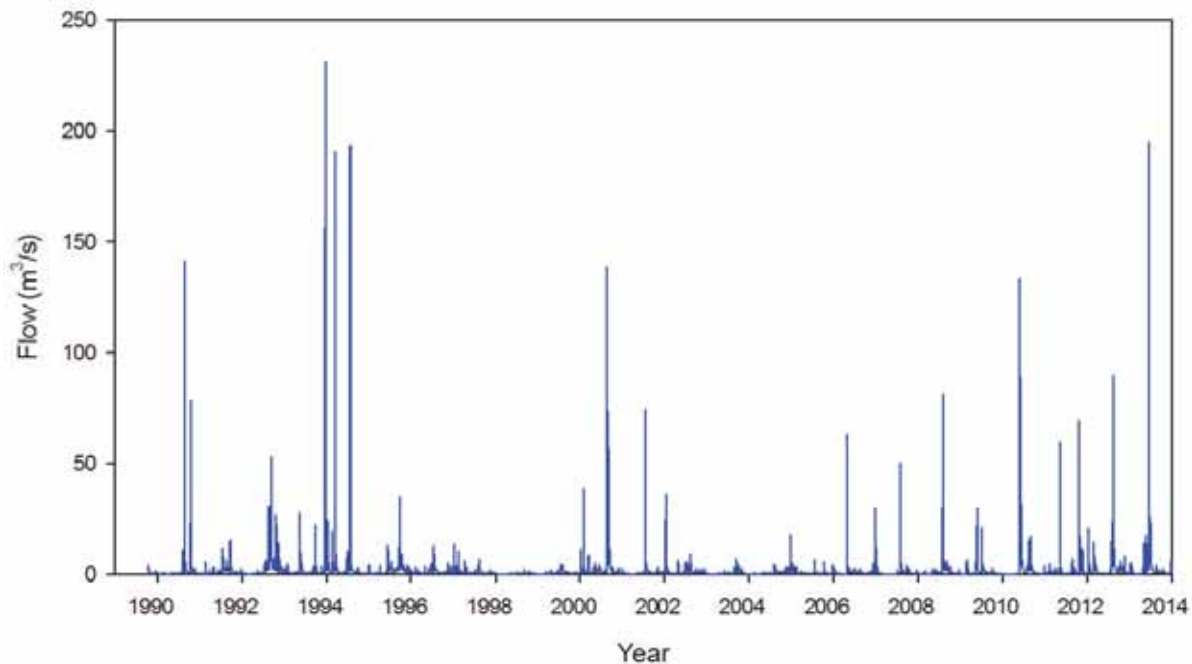
Figure 6.1 Flow (as daily means) in the Shag River/Waihemo between late 1989 and early 2014.
