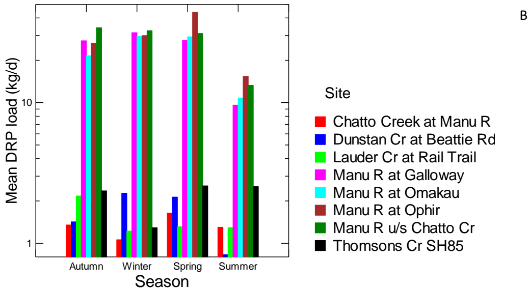
Figure 3-7: Seasonal DRP and NNN flux estimates for sites in the Manuherikia River catchment, based on data collected over 2009 to 2019. Note y-axes have a log 10 scale.
