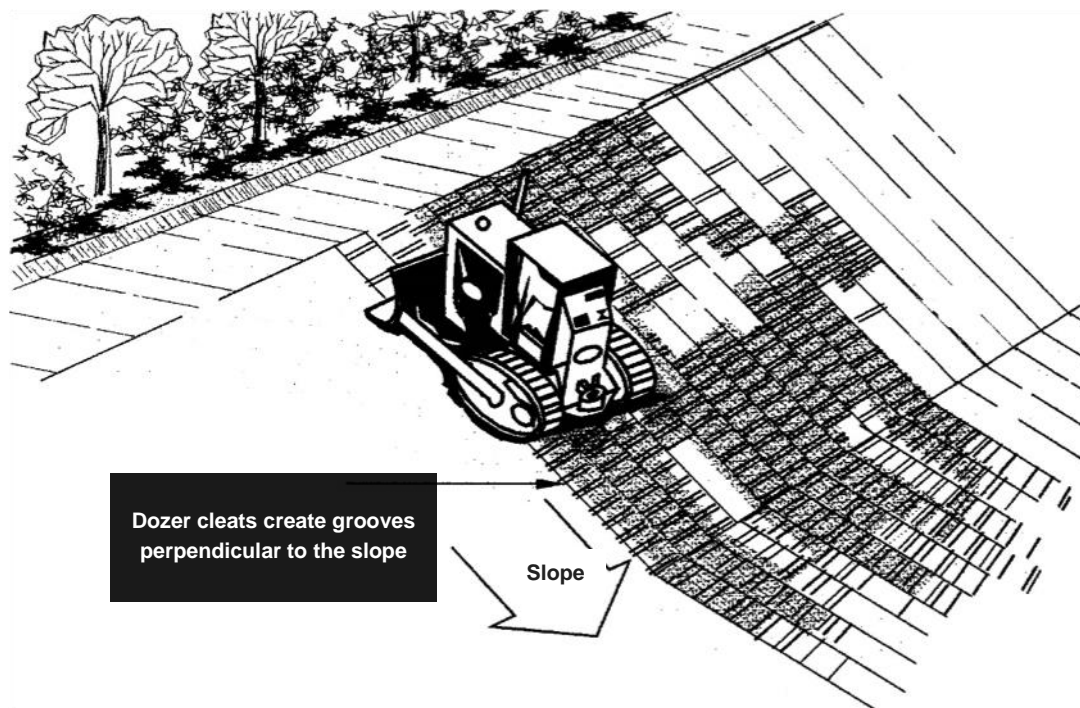
Figure 40: Surface roughening
