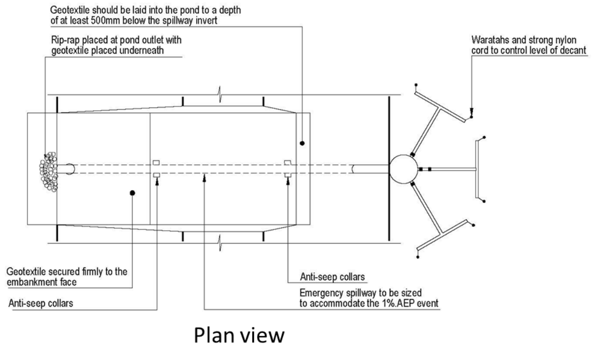
Figure 73: Sediment retention pond for 3 to 5 ha catchment
