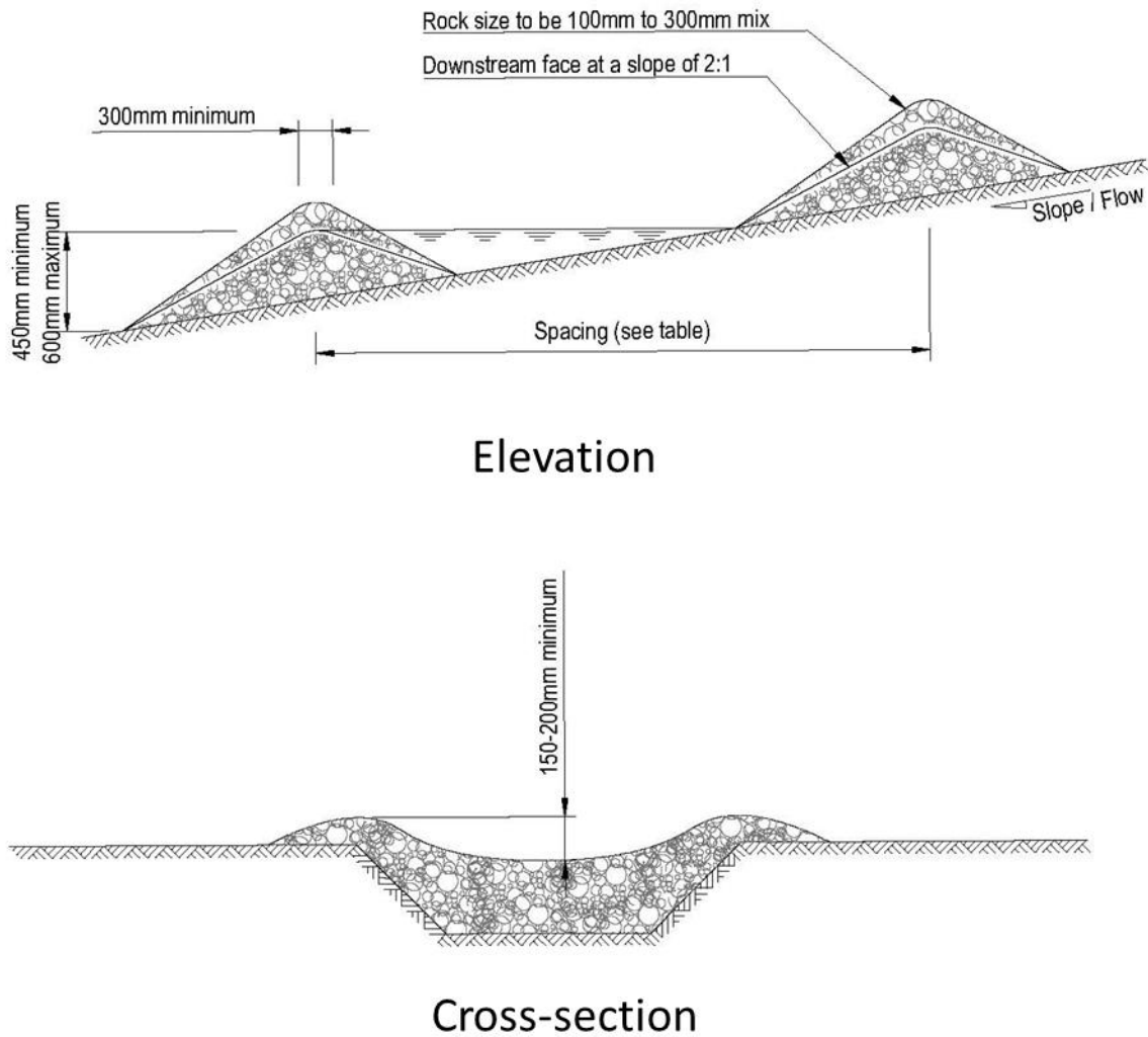
Figure 28: Rock check dam
