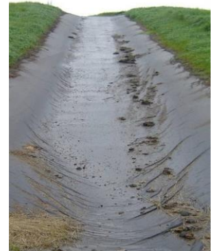
Figure 30: Geotextile lined flume
