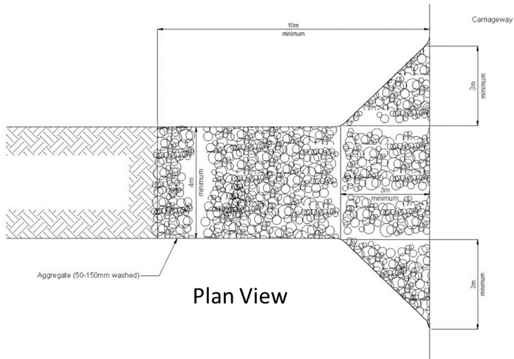
Figure 35: Stabilised entranceway
