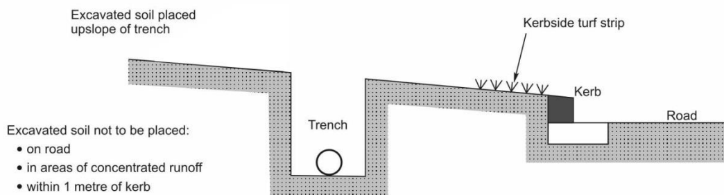
Figure 110: Typical trenching methodology
