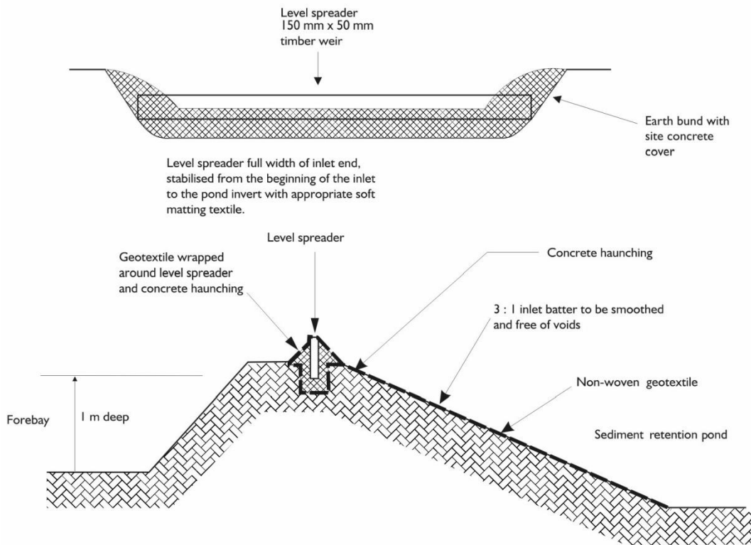
Figure 69: Level spreader
