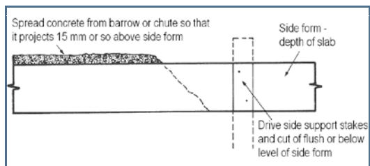
Figure 9: Placing Concrete
