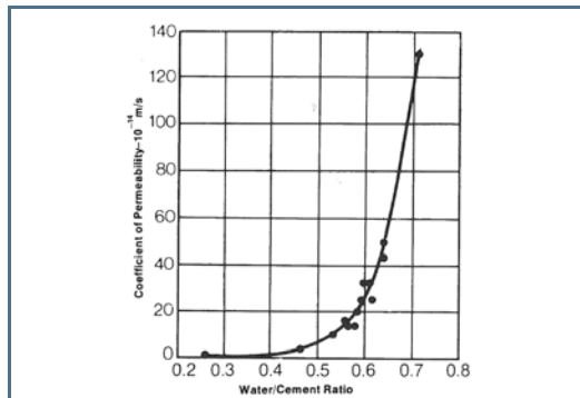
Figure 2: Relationship between permeability and water/cement ratio for mature cement pastes
