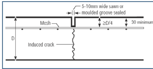
Figure 6: Tied joints
