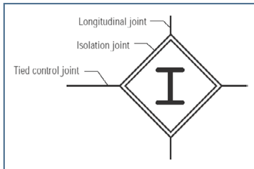
Figure 7: Isolation joint
