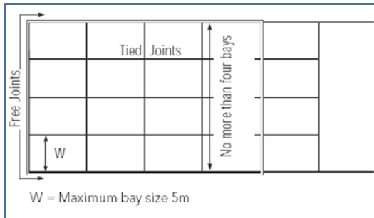
Figure 4: Joint spacing
