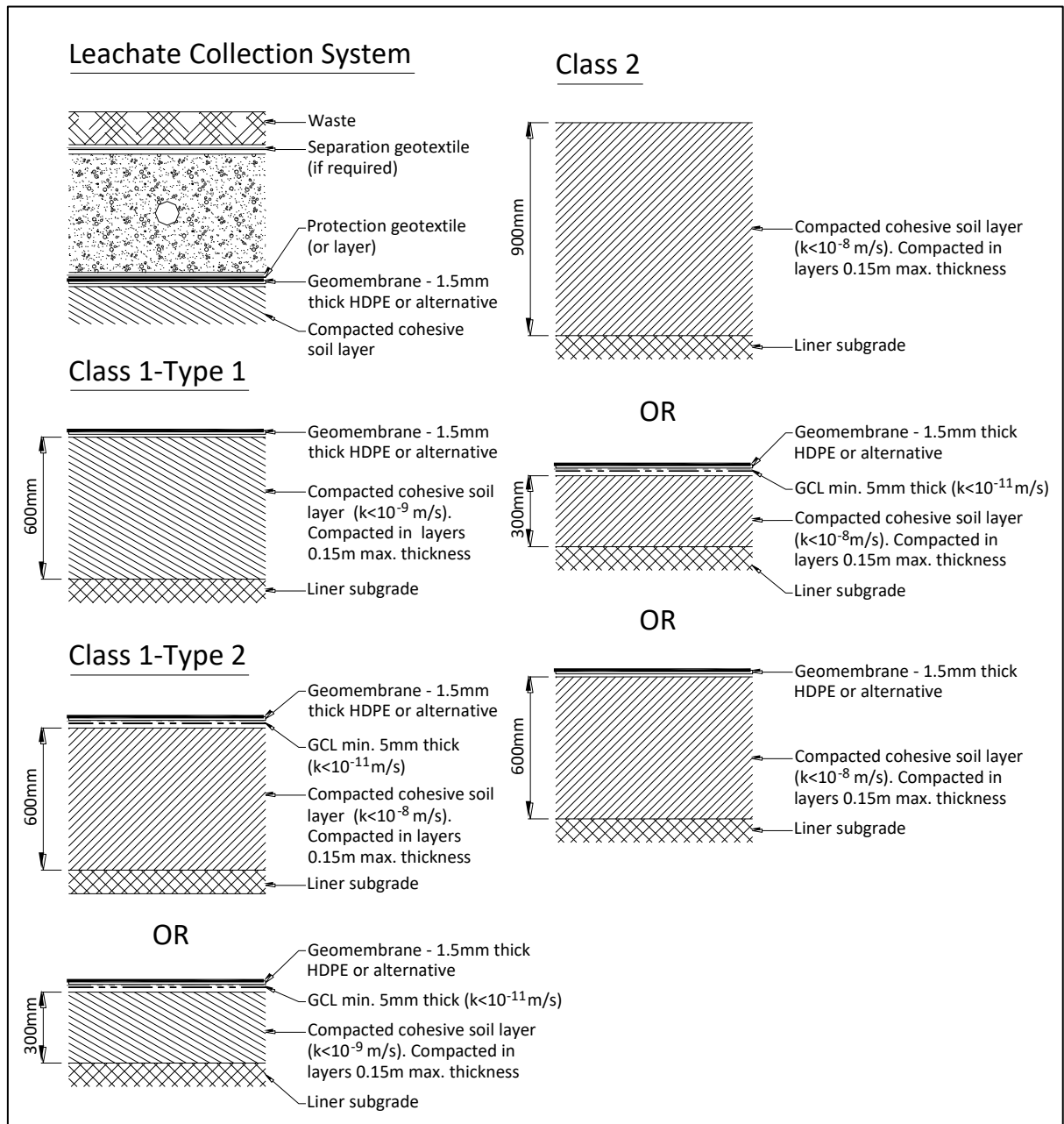
Figure 5-2 Liner Types
